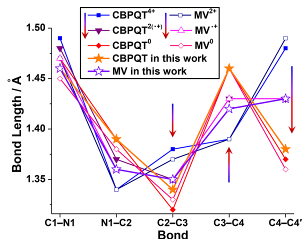
Figure 3. Comparison of bond lengths of BIPY in MV and CBPQT for \text{MVC}(\text{CBPQT})_2 with BIPY in \text{CBPQT}^{4+} , \text{CBPQT}^{2(+)} , \text{CBPQT}^0 , \text{MV}^{2+} , \text{MV}^{*+} , and \text{MV}^0 . Arrows indicate the changes in bond lengths of BIPY.
