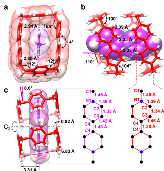
Figure 2. Crystal (super)structure of \text{MVC}(\text{CBPQT})_2 . (a) Front view showing the corner angles of CBPQT, torsional angle of BIPY in CBPQT, and [\text{C}-\text{H}\cdots\pi] interactions (pink dash lines). (b) Side view exhibiting the angles between xylene planes and CBPQT, the dihedral angle between MV and CBPQT, and [\text{H}\cdots\text{H}] interactions (blue dash lines) between two CBPQT. (c) Top view indicating the \text{C}_2 symmetrical axis and the width of CBPQT, and \pi-\pi interactions between MV and CBPQT. H, white; CBPQT, red; MV, purple. The bond lengths of BIPY in MV and CBPQT are portrayed in purple and red, respectively.
