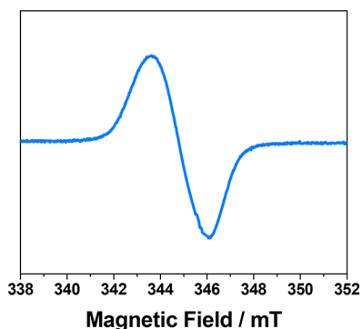
Figure 4. Solid-state continuous-wave EPR spectrum of crystals of [\text{MVC}(\text{CBPQT})_2]_3 \cdot (\text{PF}_6)_2 .
