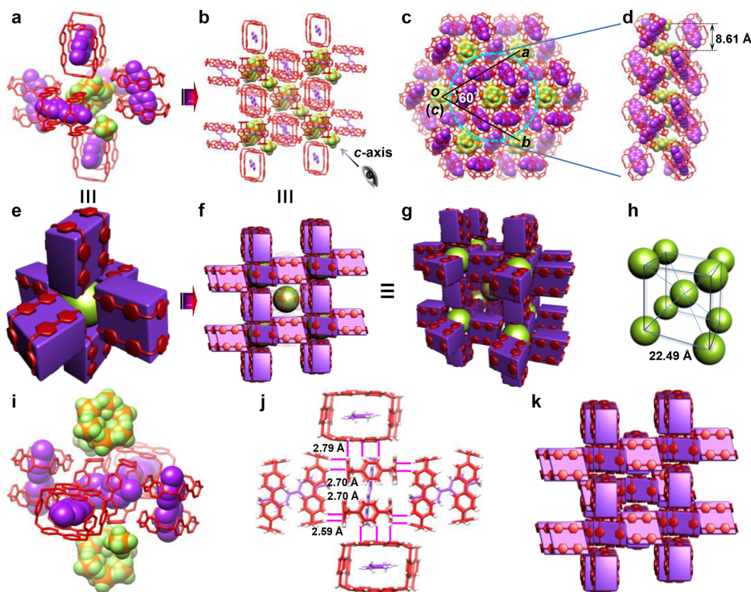
Figure 5. Crystal superstructure of [\text{MVC}(\text{CBPQT})_2]_3 \cdot (\text{PF}_6)_2 . (a) Octahedron assembled from six \text{MVC}(\text{CBPQT})_2 surrounding two \text{PF}_6^- and (e) its schematic representation. (b) Body-centered cubic superstructure assembled by adjacent octahedrons sharing \text{MVC}(\text{CBPQT})_2 as linkers and (f and g) its schematic representations. (d) Hexagonal channels packing into (c) hexagonal arrangement as viewed along the c -axis (the diagonal of the cube in panel b). (h) Schematic representation of body-centered cubic superstructure after removing all \text{MVC}(\text{CBPQT})_2 . Green balls represent \text{PF}_6^- pairs in panels e–h. (i) A representation showing that every \text{MVC}(\text{CBPQT})_2 is encircled by four \text{MVC}(\text{CBPQT})_2 and two pairs of \text{PF}_6^- . (j) 20 Complementary [\text{C}-\text{H} \cdots \pi] interactions (Figure S2) of 2.59–2.79 Å between BIPY planes and H atoms on CBPQT of adjacent \text{MVC}(\text{CBPQT})_2 . (k) Schematic representation of an extended body-centered cubic framework wherein \text{PF}_6^- pairs are omitted. CBPQT, red; MV, purple; F, green; P, yellow. H atoms in panels a–d and i and solvents are omitted.
