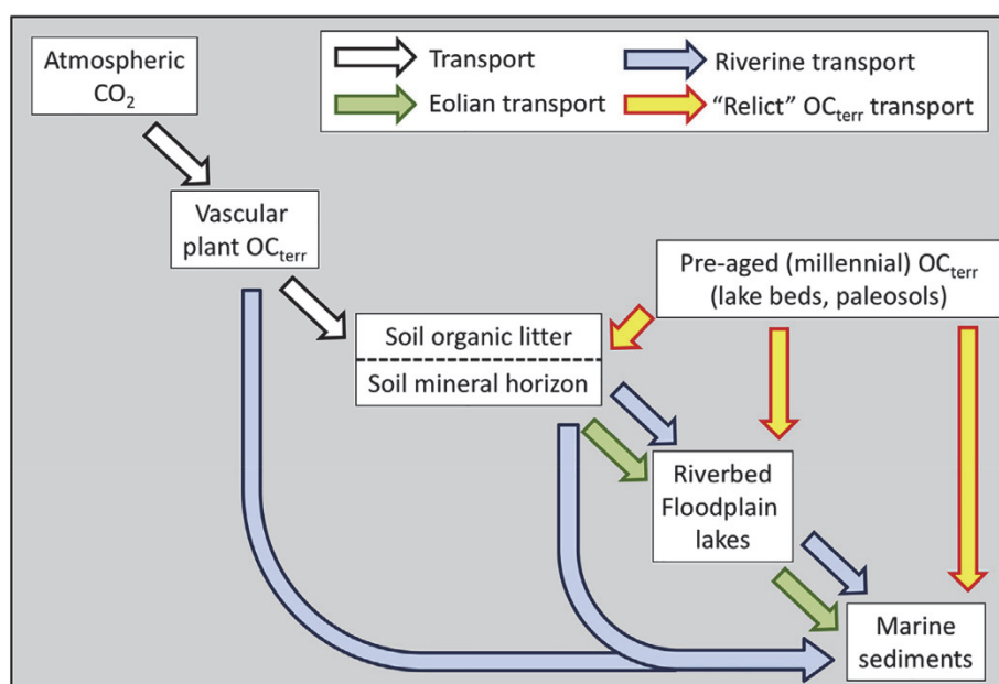
Fig. 1. Simplified schematic of potential transport pathways and intermediate storage reservoirs of terrestrial organic carbon (OC terr ) from biological source to marine sedimentary sink. Note that pre-aged OC (petrogenic or biospheric) also originates from atmospheric CO 2 and vascular plant OC but arrows are not shown here.
