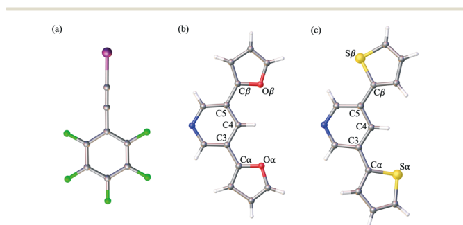
Fig. 1 Select fragment structures from the crystal structures of (a) F 5 BAI XB donor and both (b) PyrFur 2 and (c) PyrThio 2 XB acceptors. Torsional angles within each XB acceptor are defined as \tau_\alpha = C4–C3–C \alpha –Y \alpha and \tau_\beta = C4–C5–C \beta –Y \beta , where Y = O or S.
