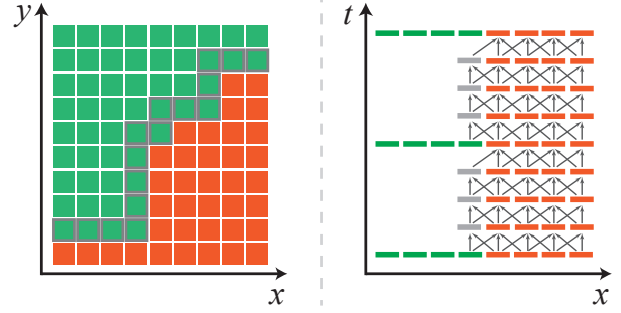
Figure 7: “Buffer blocks” in gray. The green blocks have 4\times larger \Delta t than orange blocks. Left: In this 2D example, buffer blocks (gray contour) are generated near the boundary of \Delta t change, on the side with larger \Delta t . Right: In this 1D example, buffer blocks are updated together with orange blocks. Note that they depend on only other buffer blocks and orange blocks, and they are never used to update green blocks.
