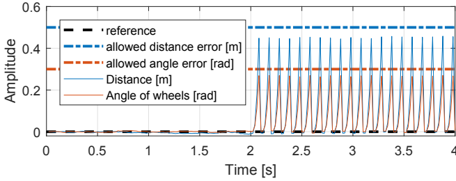
Fig. 4. Simulation of the steering control system in the presence of a stealthy attack on system sensors, with the attack starting at 2 s.
