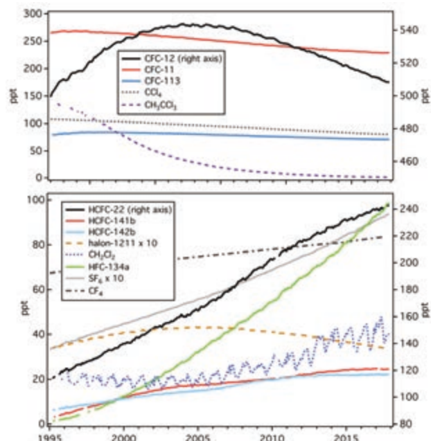
FIG. 2.47. Global mean mole fractions at Earth's surface (ppt, dry air) for several LLGHG, many of which also deplete stratospheric ozone. See Table 2.6 for the 2017 global mean mole fractions of these gases.
