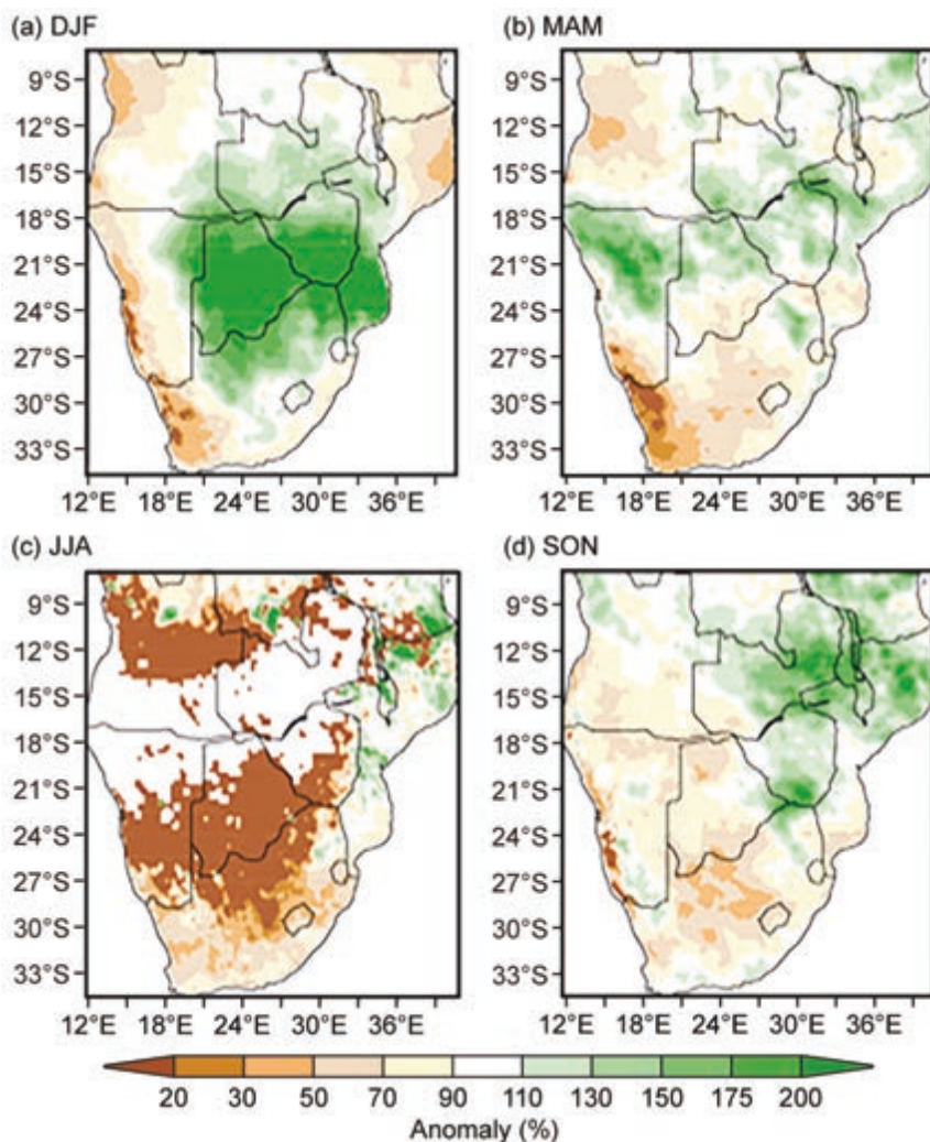
FIG. 7.28. Southern Africa seasonal total rainfall anomalies (% of normal; 1981–2010 base period) for (a) DJF 2016/17 and (b) MAM, (c) JJA, and (d) SON 2017 (Source: CHIRPS.)
