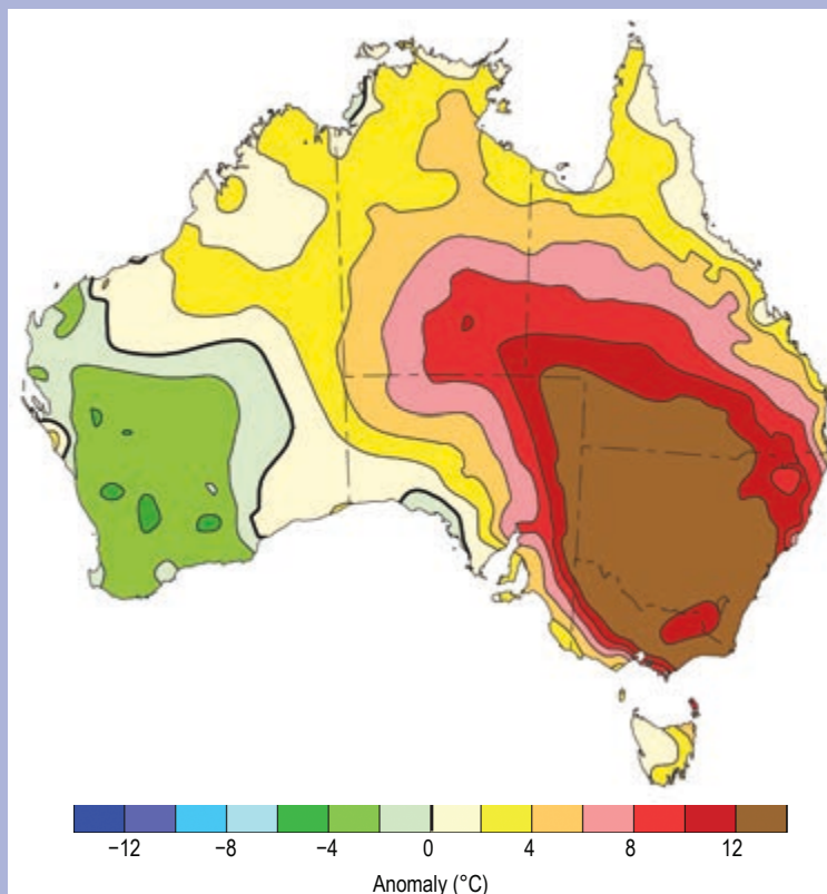
FIG. SB7.6. Maximum temperature difference (°C) from the 1981–2010 average for 23 Sep 2017. (Source: Australia Bureau of Meteorology.)
