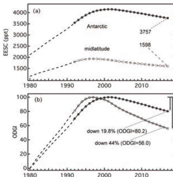
FIG. 2.48. (a) EESC (ppt) and (b) NOAA ODGI. The ODGI represents the relative mole fractions of reactive halogen in the midlatitude (open circles) and Antarctic stratosphere (closed circles) scaled such that ODGI = 100 at maximum EESC and zero in 1980. Both EESC and ODGI are derived from NOAA surface measurements of long-lived ODS (circles) or, for earlier years, WMO scenarios (dashed lines; N. Harris et al. 2014). The EESC and ODGI values from 1992 forward correspond to Jan of each year.
