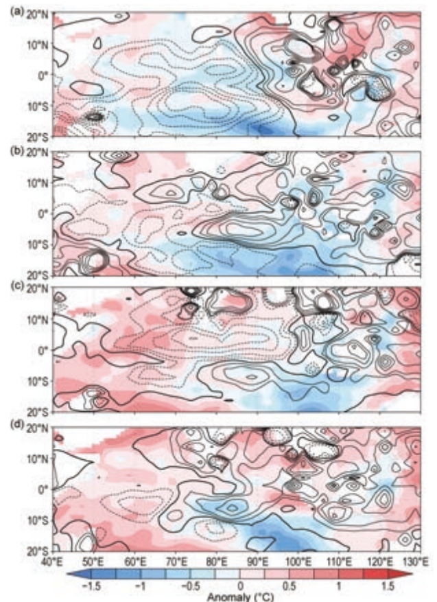
FIG. 4.41. SST (°C; colors) and precipitation (contoured at: 0, \pm 0.5 , \pm 1 , \pm 2 , \pm 3 , \pm 4 , and \pm 5 mm day -1 ). Solid/dashed lines denote positive/negative values, and thick solid lines indicate the zero contour) anomalies during (a) Dec 2016–Feb 2017, (b) Mar–May 2017, (c) Jun–Aug 2017, and (d) Sep–Nov 2017. Anomalies were calculated relative to 1982–2017. [Sources: NOAA OISST (Reynolds et al. 2002) and monthly GPCP precipitation analysis (available at http://precip.gsfc.nasa.gov/ ).]
