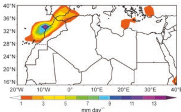
FIG. 7.21. Northern Africa 2017 rainfall rate anomalies (mm day -1 ; 1981–2010 base period) over 21–24 Feb. (Source: NOAA/NCEP.)
