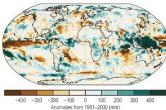
(k) Maximum 1 Day Precipitation Amount (Rx1day)
