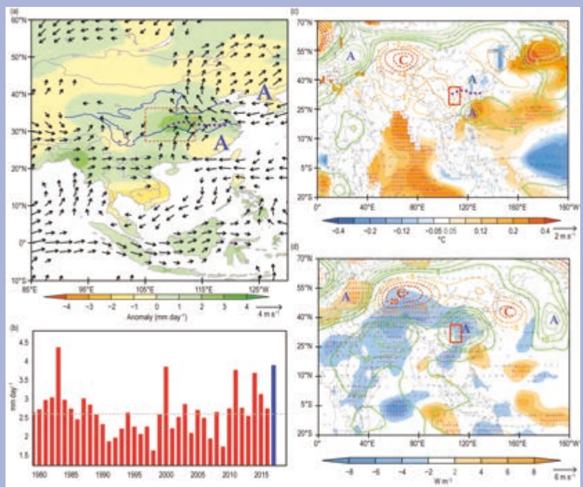
FIG. SB7.4. (a) Precipitation (shading; mm day −1 ) and 850-hPa wind (vector; m s −1 ) anomalies in Sep and Oct 2017. Only winds with speeds >1 m s −1 are shown. (b) Year-to-year time series of the WCAR (red bars; mm day −1 ). 2017 is blue bar. Gray dashed line is the 1981–2010 climatological mean. (c) Wind (vectors; m s −1 ), geopotential height (contours; gpm) at 850-hPa, and SST (°C) fields regressed onto the WCAR index. (d) as in (c) but for 200-hPa wind, geopotential height, and OLR (W m −2 ) fields. Only winds significant at the 95% confidence level are shown, and the SST and OLR significant at 95% confidence level are marked by red dots. “A (C)” denotes the anticyclonic (cyclonic) anomaly. Red box indicates the key region of WCAR, dashed purple line marks the horizontal trough.
