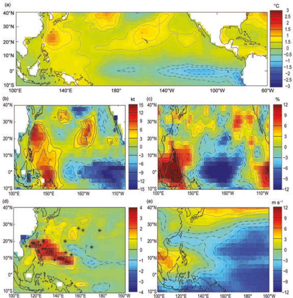
FIG. 4.30. (a) SST anomalies (°C) for Jul–Oct (JASO) 2017. (b) PI anomalies (kt) in JASO 2017. (c) Relative humidity 600-hPa relative humidity anomalies (%) in JASO 2017. (d) GPI anomalies in JASO 2017. First positions of storms in JASO 2017 are marked with an asterisk. (e) Zonal winds in JASO 2017 (positive contours are shown in solid lines, negative contours in dash dotted lines and the zero contour in a dotted line) [Source: atmospheric variables: NCEP/NCAR Reanalysis data (Kalnay et al. 1996); SST (Smith et al. 2008).]
