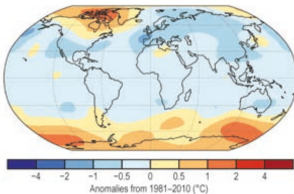
(f) Lower Stratospheric Temperature
