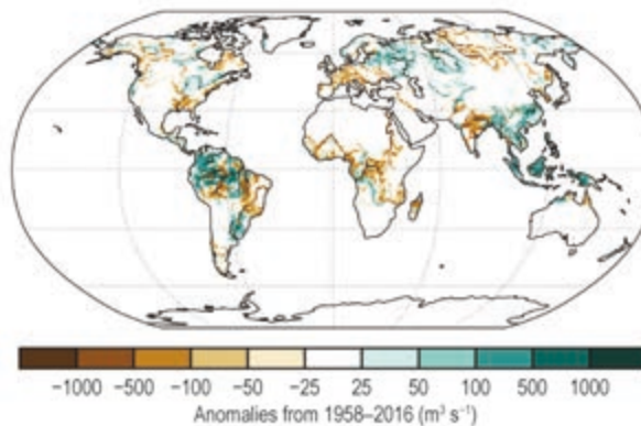
(m) River Discharge
