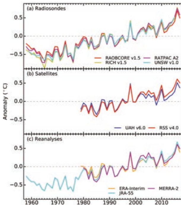
FIG. 2.7. Anomalies of global mean LTT (°C; 1981–2010 base period): (a) radiosondes, (b) satellites, and (c) reanalyses.
