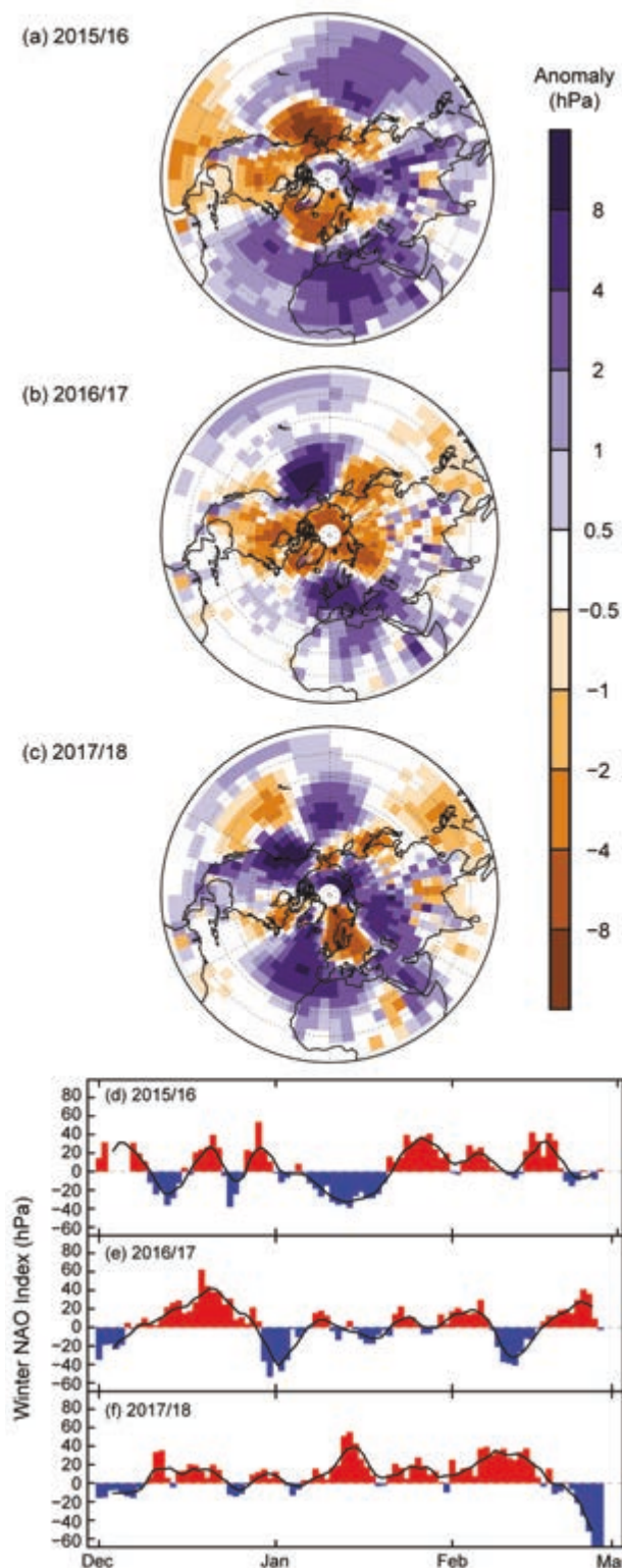
FIG. 2.36. Boreal winter sea level pressure anomalies (hPa; 1981–2010 base period) averaged over Dec–Feb for (a) 2015/16, (b) 2016/17, and (c) 2017/18. NAO daily time series (hPa) for winter (d) 2015/16, (e) 2016/17, and (f) 2017/18. The 5-day running mean is shown by the solid black line. The data are from HadSLP2r (Allan and Ansell 2006).
