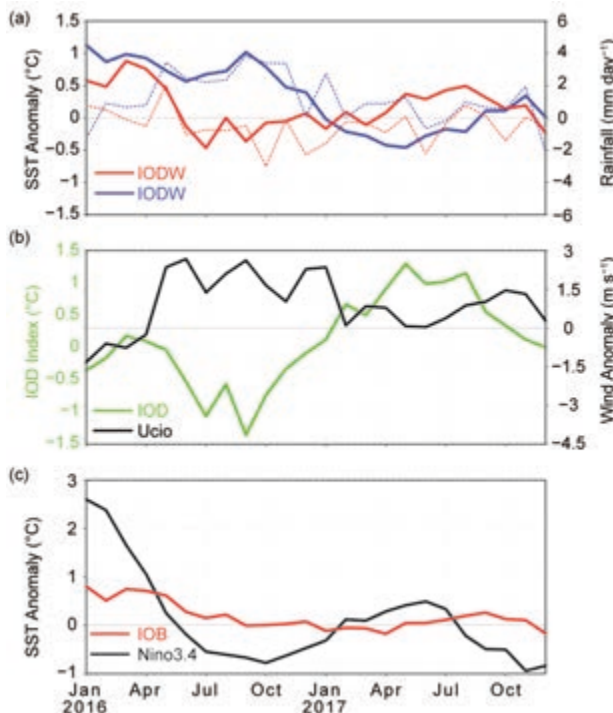
FIG. 4.40. (a) Monthly anomalies of SST (°C; solid lines) and precipitation (mm day -1 ; dashed lines) in the eastern pole (IODW; 10°S–0°, 90°–110°E; blue lines) and the western pole (IODW; 10°S–10°N, 50°–70°E; red lines) of the IOD. (b) As in (a), but for the IOD index (measured by the SST difference between IODW and IODE, green line) and surface zonal wind anomaly (m s -1 ) in the central equatorial IO (Ucio; 5°S–5°N, 70°–90°E; black line). (c) As in (a), but for the SST anomalies in the Niño-3.4 region (5°S–5°N, 190°–240°E; black line) and the tropical IO (IOD; 20°S–10°N, 40°–120°E; red line). Anomalies are relative to the 1982–2017 base period. [Sources: NOAA OISST (Reynolds et al. 2002); monthly GPCP precipitation analysis (available at http://precip.gsfc.nasa.gov/ ); and JRA-55 atmospheric reanalysis (Ebata et al. 2011).]
