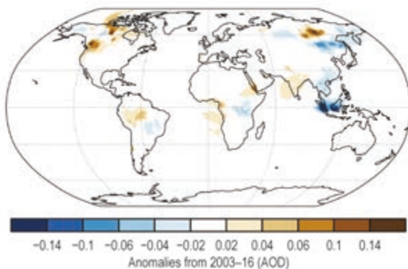
(ab) Biomass Burning Aerosol
