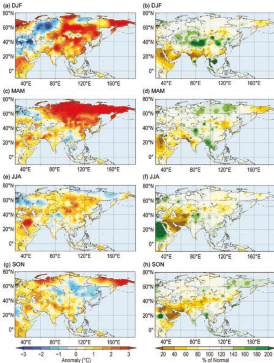
FIG. 7.40. Seasonal mean surface temperature anomalies (°C, left column) and seasonal precipitation (% of normal, right column) over Asia in 2017 for (a), (b) winter; (c), (d) spring; (e), (f) summer; and (g), (h) autumn. All relative to 1981–2010. (Source: Japan Meteorological Agency)
