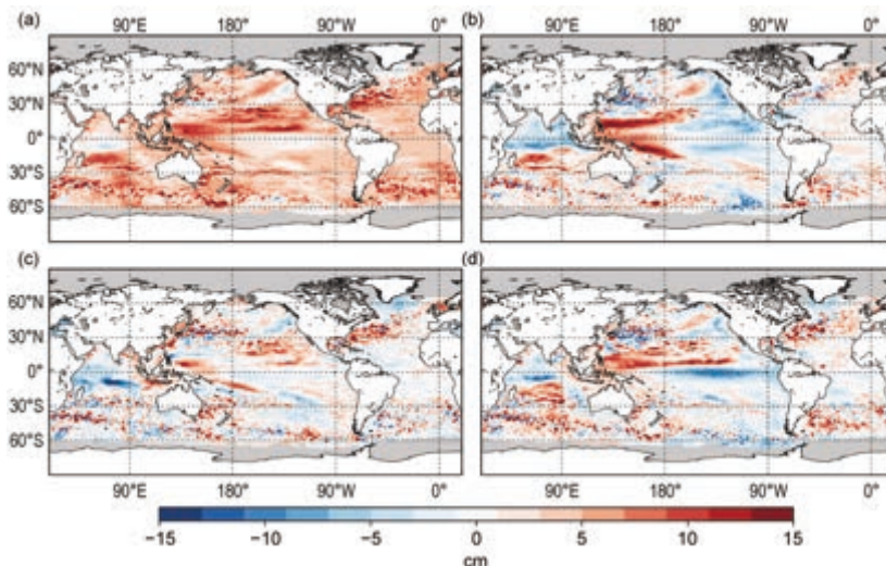
FIG. 3.16. (a) Annual average sea level anomaly during 2017 relative to the average sea level at each location during 1993–2017. (b) Average 2017 sea level anomaly minus 2016. (c) Average sea level anomaly during Dec 2016–Feb 2017 (DJF) relative to the DJF average during 1993–2017. (d) Same as (c), but for Sep–Nov 2017. GMSL was subtracted from (c) and (d) to emphasize regional, non-secular change. Altimetry data were obtained from the gridded, multimission product maintained by the Copernicus Marine and Environment Monitoring Service (CMEMS).
