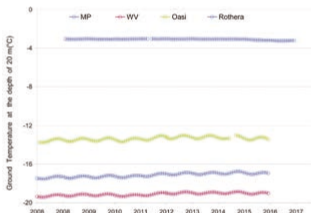
FIG. 2.13. Observed borehole temperatures (°C) in Antarctica at 20-m depth (monthly means): WV = Wright Valley; MP = Marble Point; Oasi in continental Antarctica; and Rothera in maritime Antarctica. (Source: Insubria Permafrost Database.)
