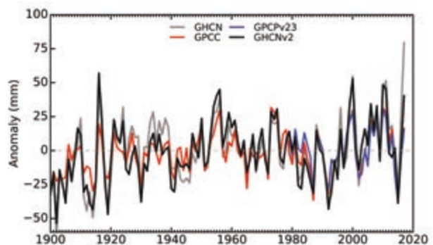
FIG. 2.22. Globally averaged precipitation anomalies (mm yr -1 ) over land areas relative to the 1961–90 base period (except GPCP v2.3, which is 1981–2000).
