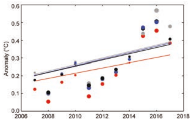
FIG. 2.2. Annual global temperature anomalies ( ^{\circ}\text{C} ; displayed as dots) from 2007–17. Lines represent the linear trends over the 1975–2017 period, while the size of the dot represents the trend residuals. The black, gray, red, and blue colors represent the NOAA GlobalTemp, NASA GISS, JMA, and HadCRUT datasets, respectively.
