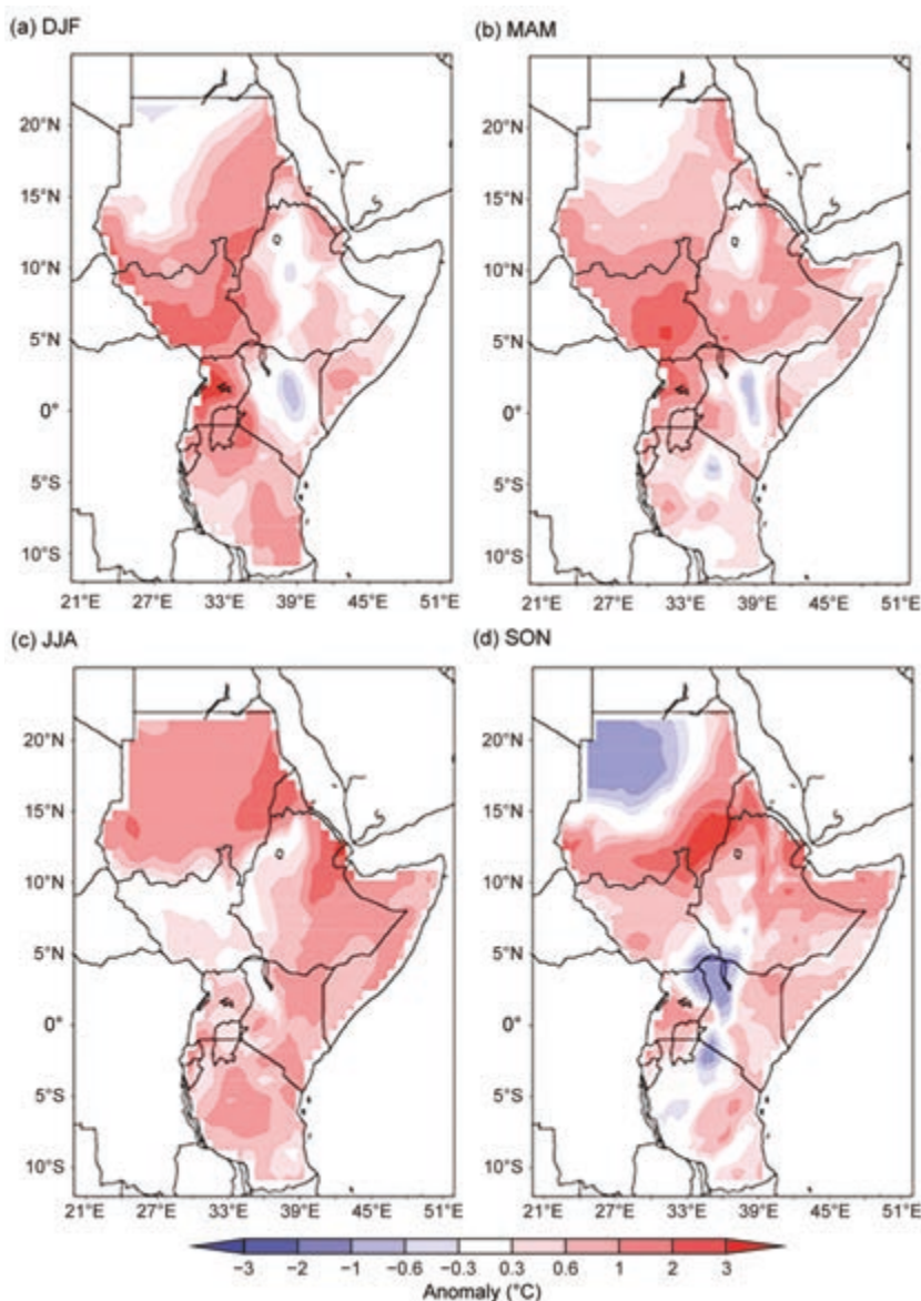
FIG. 7.24. Eastern Africa seasonally averaged mean temperature anomalies (°C; 1981–2010 base period) for (a) DJF 2016/17 and (b) MAM, (c) JJA, and (d) SON 2017 (Source: ERA-Interim.)
