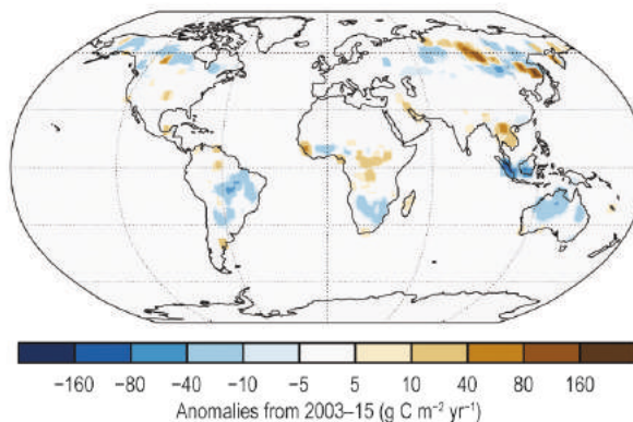
(ad) Carbon Emissions from Biomass Burning
