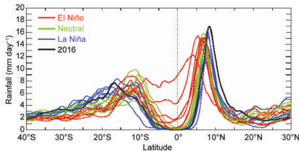
FIG. 4.14. CMORPH rainfall rate ( \text{mm day}^{-1} ) for Oct–Dec quarters, for each year 1998 to 2016, averaged over the longitude sector 180^{\circ} – 150^{\circ}\text{W} . The cross-sections are color-coded according to NOAA’s ONI, except for 2016 (a La Niña quarter) shown in black.
