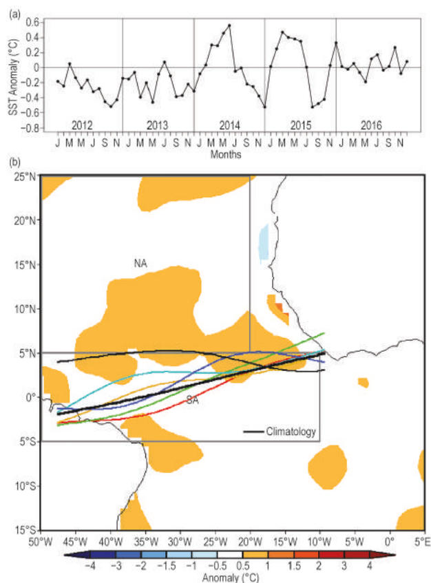
FIG. 4.17. (a) Monthly OISST (Smith et al. 2008) anomaly time series averaged over the South American sector (SA region, 10°–50°W, 5°S–5°N) minus the SST anomaly time series averaged over the North Atlantic sector (NA region, 20°–50°W, 5°–25°N) for the period 2012–16, forming the Atlantic index. The positive phase of the index indicates favorable conditions for enhanced Atlantic ITCZ activity. (b) Atlantic ITCZ position inferred from OLR (Liebmann and Smith 1996) during Apr 2016. The colored thin lines indicate the approximate position for the six pentads of the month. The black thick line indicates the Atlantic ITCZ climatological position for April. The SST anomalies for Apr 2016 based on the 1982–2015 climatology are shaded (°C). The two boxes indicate the areas used for the calculation of the Atlantic index in (a).
