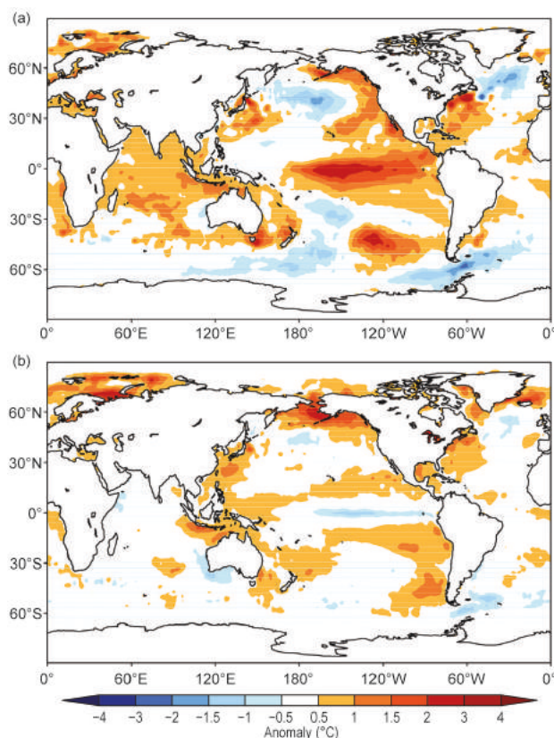
FIG. 4.15. Spatial distribution of 2016 average global SST anomalies (°C; Reynolds et al. 2002) for (a) Jan–Apr and (b) May–Dec.
