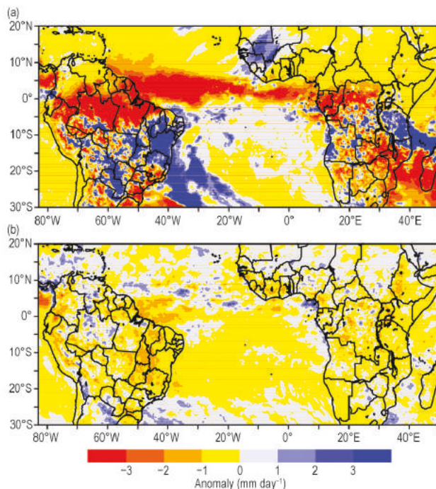
FIG. 4.16. Observed 2016 precipitation anomalies for (mm day -1 ) tropical and subtropical South America during (a) Jan and (b) Feb–Dec 2016. Anomalies calculated based on a 1998–2015 climatology derived from CMORPH (Joyce et al. 2004).
