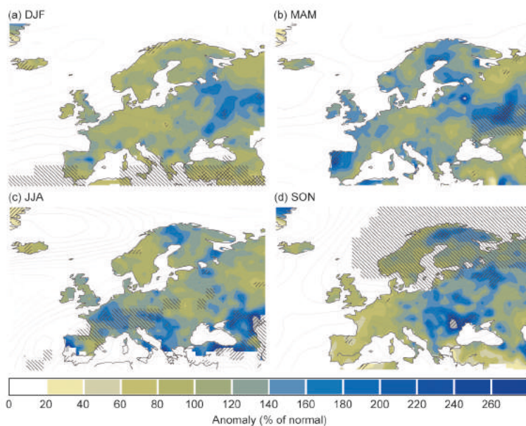
FIG. 7.38. Seasonal anomalies for 2016 (1981–2010 base period) of sea level pressure (hPa, contours) and seasonal precipitation anomalies (% of normal, shading) from NCAR–NCEP reanalysis for (a) DJF, (b) MAM, (c) JJA, and (d) SON. Left hatches indicate where the anomaly at sea level pressure is significant at the 5th or 95th percentile. Right hatches show the same conditions for seasonal precipitation. White areas have received either less than 20% of normal or below 15 mm seasonal precipitation. Negative sea level pressure anomalies are indicated by dashed contours. Black areas indicate regions where data have been inadvertently omitted from the figure. Please note the base period used here is different from that used in Fig. 7.37. (Source: NOAA/ESRL Physical Sciences Division, www.esrl.noaa.gov/psd .)
