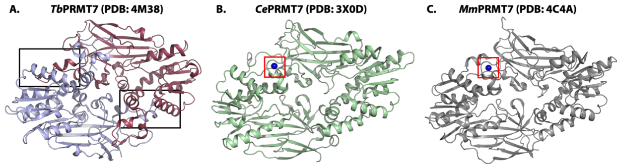
Figure 3. Overall Crystal structures of PRMT7 from a protist ( Trypanosoma brucei , Tb PRMT7), a nematode worm ( Caenorhabditis elegans , Ce PRMT7), and a mammal ( Mus musculus , Mm PRMT7). A) Crystal structure of Tb PRMT7 (PDB: 4M38) as a homodimer; one monomer is colored raspberry and the other light blue. The dimerization arms are indicated in the black boxes. B) Crystal structure of Ce PRMT7 (PDB: 3X0D) in pale green; the Zn-finger like domain is boxed in red and the \text{Zn}^{2+} ion is shown as a blue sphere. C) Crystal structure of Mm PRMT7 (PDB: 4C4A) in gray; the Zn-finger like domain is boxed in red and the \text{Zn}^{2+} ion is shown as a blue sphere.
