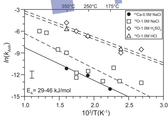
Fig. 8. The natural log of the rate constants, \ln(k_{\text{AnH}}) , in units of reciprocal time ( \text{s}^{-1} ), as a function of temperature. The \ln(k_{\text{AnH}}) data are determined by linear regression of the fractional approach to complete mixing versus time by utilization of 1st order rate law (Table 2). The activation energy, E_A , indicative of Ca isotope exchange between anhydrite and dissolved \text{Ca}^{2+} at hydrothermal conditions is determined from the slope of the linear regression of the \ln(k_{\text{AnH}}) data versus 10^3/T(\text{K}) , amounting to approximately 46 kJ/mol. The magnitude of the E_A is consistent in magnitude with the exchange mechanism of dissolution and precipitation (i.e. recrystallization) and with previously calculated activation energies for oxygen isotope exchange reactions between sulfate minerals and dissolved constituents at similar experimental conditions, 29–46 kJ/mol (Chiba et al., 1981).
