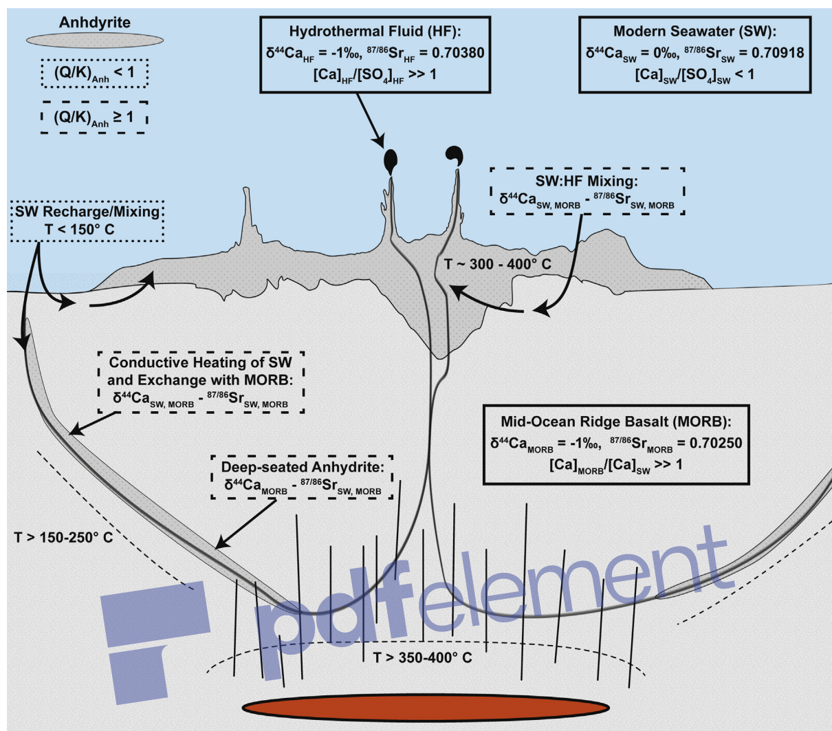
Fig. 1. Schematic diagram of the different zones of anhydrite at and below the seafloor, as indicated by the grey speckle areas. Dissolution of anhydrite, (Q/K)_{\text{Anh}} < 1 (dotted rectangle), occurs at low temperature, < 150^\circ\text{C} , as a result of pervasive seawater mixing and subsequent cooling of the hydrothermal mound at and below the seafloor. Anhydrite precipitation, (Q/K)_{\text{Anh}} \geq 1 (dashed rectangles), occurs at temperatures > 150^\circ\text{C} and is a result of conductive heating of seawater and/or mixing with high temperature hydrothermal fluid. The chemical and isotopic composition of the sources of Ca, Sr, and \text{SO}_4 recorded by anhydrite upon formation are described by the solid rectangles. Each zone of anhydrite precipitation corresponds to a distinct Ca and Sr isotope compositions as a consequence of different physiochemical processes taking place in the subseafloor, such as conductive heating of seawater upon recharge of seawater into the hydrothermal system versus mixing of hydrothermal fluid, such as seawater. The anhydrite formed and recovered from the TAG MOR hydrothermal system, used in this study, is representative of the zone of anhydrite precipitation at and directly below the active sulfide mound at the seafloor, as a consequence of significant mixing of conductively heated seawater with high temperature end-member hydrothermal fluids.
