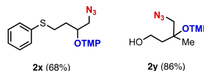
Scheme 9. Expanded Substrate Scope to Include Oxidatively Labile Functional Groups
