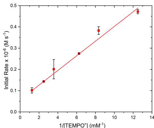
Figure 10. Plot of initial rates versus concentration of \text{TEMPO}^\bullet for the reaction between adduct I ( \text{TEMPO}^+\text{ClO}_4^- + \text{TBAN}_3 ) and alkene 11 , showing inverse first-order rate dependence on [\text{TEMPO}^\bullet] . Error bars represent the standard deviation of three independent measurements. The curve depicts an unweighted least-squares fit to the function f(x) = ax^{-1} + b : a = 0.0345 \pm 0.0008 ; b = 0.057 \pm 0.002 ; R^2 = 0.998 .
