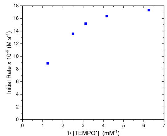
Figure 11. Plot of initial rates versus concentration of \text{TEMPO}^\bullet for the reaction between adduct I ( \text{TEMPO}^+\text{ClO}_4^- + \text{TBAN}_3 ) and alkene 11 (50 mM). Saturation kinetics were observed when \text{TEMPO}^\bullet concentration is less than 0.25 mM.
