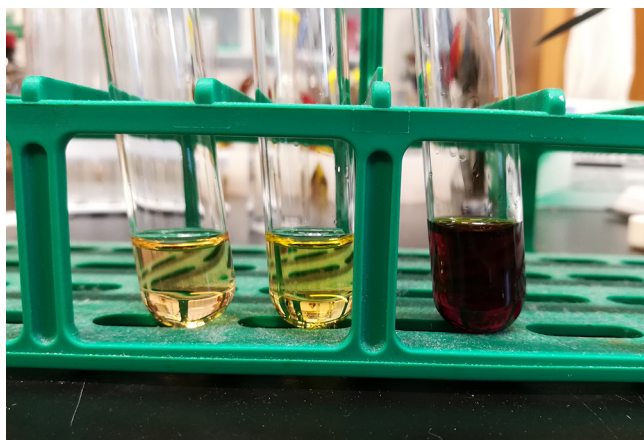
Figure 4. Color of the MeCN solution of TEMPO–N 3 adduct (right) in comparison to TEMPO• (left) and TEMPO + (center).
