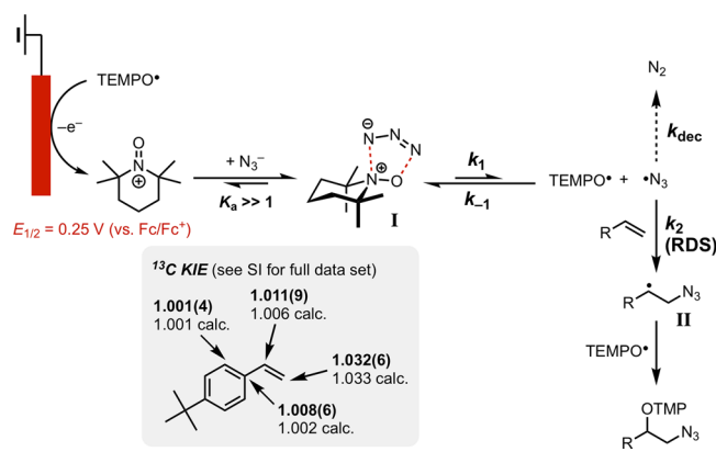
Scheme 8. Mechanism of the Electrochemical Azidooxygenation Reaction
