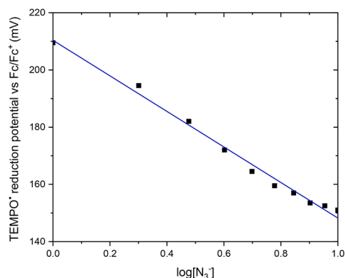
Figure 2. Cyclic voltammograms of \text{TEMPO}^\bullet in the presence of \text{N}_3^- (top), showing a Nernstian dependence of the reduction potential on [\text{N}_3^-] (bottom). The curve depicts a least-squares fit to the function f(x) = ax + b ; a = -62 \pm 2 ; b = 210 \pm 2 ; R^2 = 0.990 .
