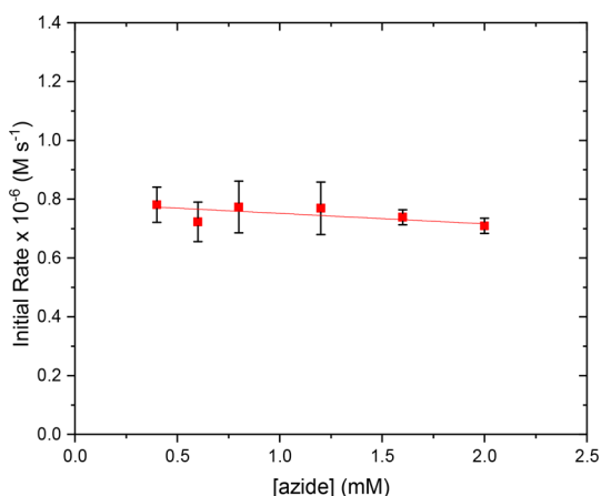
Figure 9. Plot of initial rates versus concentration of \text{N}_3^- for the reaction between adduct I ( \text{TEMPO}^+\text{ClO}_4^- + \text{TBAN}_3 ) and alkene 11 , showing zero-order rate dependence on [\text{N}_3^-] . Error bars represent the standard deviation of three independent measurements. The curve depicts an unweighted least-squares fit to the function f(x) = ax + b : a = -0.04 \pm 0.01 ; b = 0.78 \pm 0.02 ; R^2 = 0.63 .
