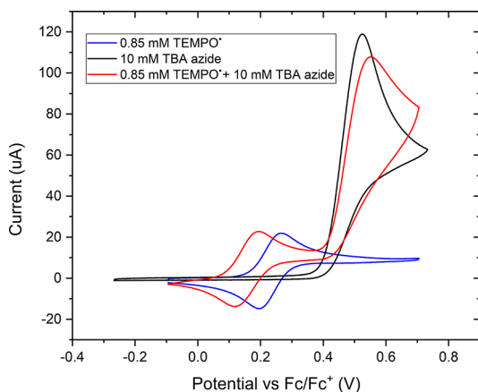
Figure 1. Cyclic voltammograms of \text{TEMPO}^\bullet , \text{N}_3^- , and their mixture.
