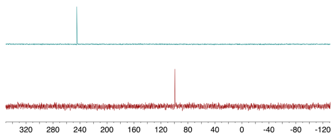
Figure 7. NMR spectra of the TEMPO-N 3 complex in MeCN (top) and NaN 3 in D 2 O (bottom).
