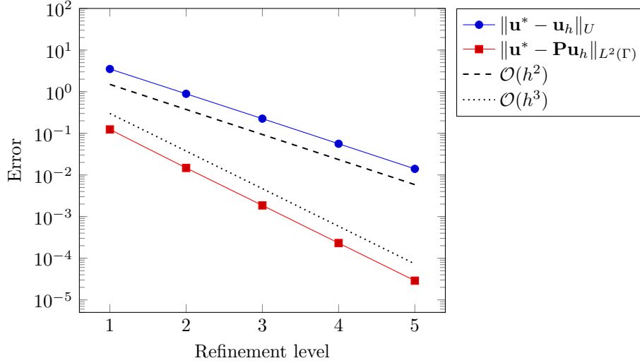
Fig. 7.9: Discretization errors for planar \Gamma , k = 2 , l = 1 and \rho = \tilde{\rho} = h .
