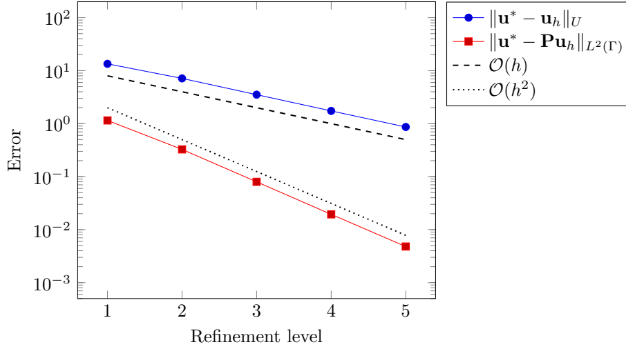
Fig. 7.8: Discretization errors for planar \Gamma , k = l = 1 and \rho = \tilde{\rho} = h .
