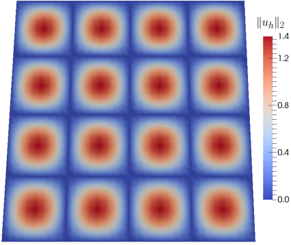
Fig. 7.6: Numerical solution on the plane for k = l = 1 , \rho = \tilde{\rho} = h and refinement level \ell = 3 .
