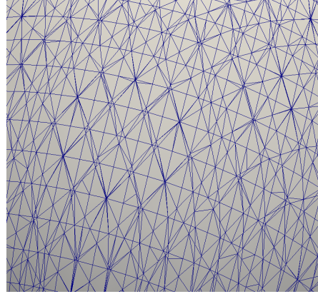
Fig. 7.2: Detail of the surface triangulation \Gamma_h of the sphere for refinement level \ell = 4 .
