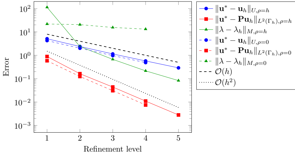
Fig. 7.5: Error norms for the sphere and k = l = 1 with \rho = \tilde{\rho} = h and \rho = \tilde{\rho} = 0 .
