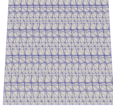
Fig. 7.7: Surface triangulation for refinement level \ell = 1 .
