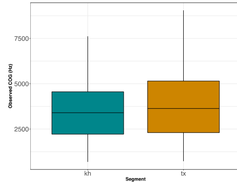
Figure 4. Observed CoG by Segment.
