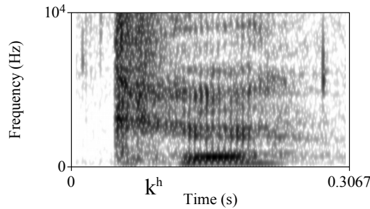
Figure 2. Spectrogram of ké from Lemuel, a 46-year-old man. VOT=71ms; CoG=2495Hz.
