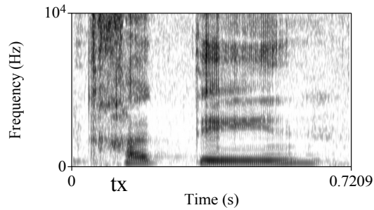
Figure 1. Spectrogram of tádiin from Annie, a 75-year-old woman. VOT= 88ms; CoG=5016Hz.
