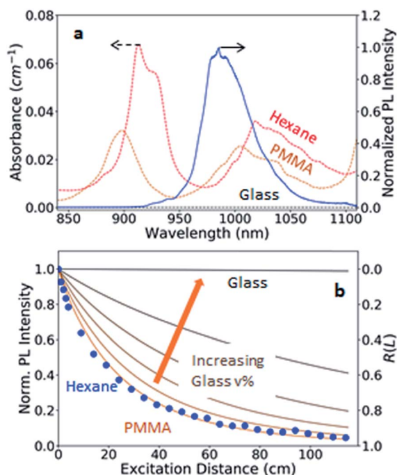
Fig. 4 (a) Absorption spectrum of hexane (red), a representative PMMA sample (orange), and Schott optical-quality glass (black) overlaid with the normalized PL spectrum of Yb 3+ :CsPbCl 3 NCs (blue). The PMMA spectrum was obtained by subtracting experimental spectra measured for two samples with different thickness to eliminate surface reflection and scattering effects. (b) Normalized PL intensity of Yb 3+ :CsPbCl 3 NCs in hexane as a function of excitation distance in a 120 cm-long 1D LSC (blue dots). The curves plot absorption probabilities for the Yb 3+ :CsPbCl 3 NC PL waveguided through glass (black) and PMMA (orange) calculated using eqn (1). The intermediate traces show the absorption probabilities in hypothetical mixed PMMA/glass waveguides with volume percentages increasing from 0% to 100% by increments of 20%.
