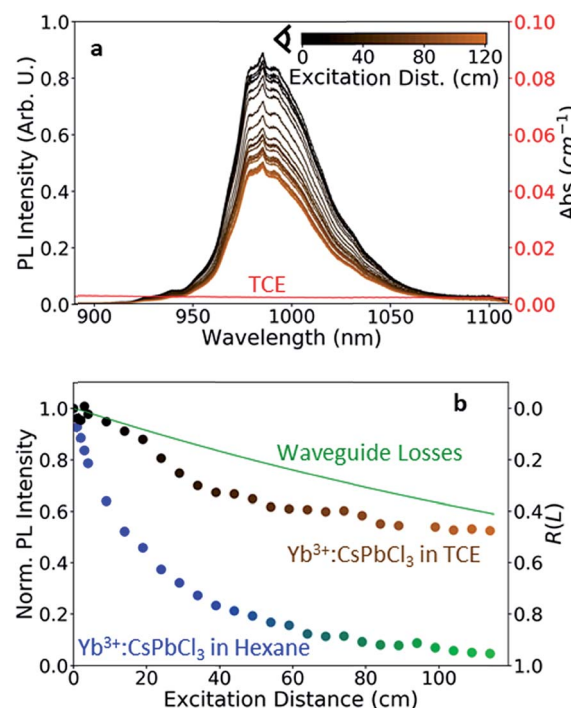
Fig. 3 (a) PL intensity of \text{Yb}^{3+}:\text{CsPbCl}_3 NCs suspended in tetrachloroethylene (TCE) from the 1D LSC experiment plotted from low excitation distances to high excitation distance with the corrected absorption spectrum of TCE. (b) Integrated normalized PL intensity of \text{Yb}^{3+}:\text{CsPbCl}_3 NCs plotted as a function of excitation distance for solutions in hexane with an \text{OD}_t \sim 0.075 \text{ mm}^{-1} (blue-green) and in TCE with an \text{OD}_t \sim 0.075 \text{ mm}^{-1} (black-brown). The green line is the experimentally determined performance limit of the 1D LSC. The analytical atomic \text{Yb}^{3+} concentration for these NCs was 4.6% and the PLQY was 138% in hexane and 71% after transfer to TCE.
