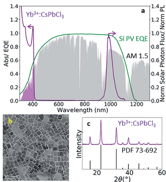
Fig. 1 (a) Absorption and normalized PL spectra of \text{Yb}^{3+}:\text{CsPbCl}_3 NCs (purple) plotted with the EQE of a NIR enhanced Si HIT PV (green) and the AM 1.5 solar spectrum (shaded area). Spectra were collected at room temperature. (b) TEM and (c) XRD data for a representative sample of \text{Yb}^{3+}:\text{CsPbCl}_3 NCs.
