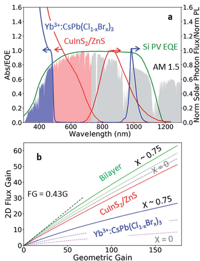
Fig. 6 (a) Absorption and normalized PL spectra of Yb 3+ :CsPb(Cl 1-x Br x ) 3 NCs with x \sim 0.75 (blue) and CuInS 2 /ZnS NCs (red) overlaid with the AM 1.5 solar spectrum (shaded area) and the external quantum efficiency (EQE) of a NIR enhanced Si HIT PV (green). (b) Projected 2D flux gain of a Yb 3+ :CsPb(Cl 1-x Br x ) 3 NC LSC (purple to blue gradient), a CuInS 2 /ZnS NC LSC (red), and the monolithic bilayer device shown in Fig. 5a (black to green). The absorption onset of the Yb 3+ :CsPb(Cl 1-x Br x ) 3 NCs is varied linearly from 412 \text{ nm} to 488 \text{ nm} for the three plotted traces.
