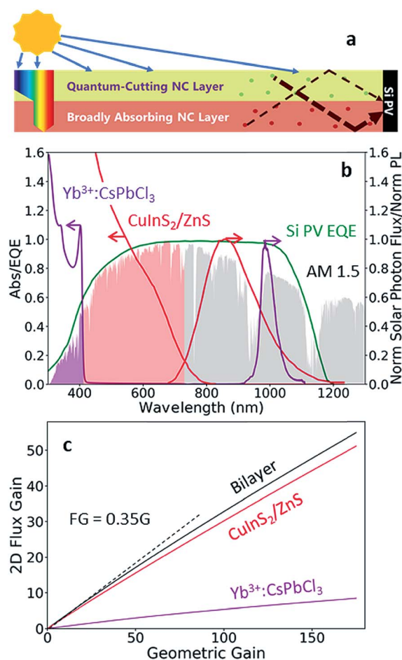
Fig. 5 (a) Schematic of the proposed monolithic bilayer LSC. The top layer contains quantum-cutting NCs (e.g., \text{Yb}^{3+}:\text{CsPb}(\text{Cl}_{1-x}\text{Br}_x)_3 NCs) and the bottom layer contains broadly absorbing NCs (e.g., \text{CuInS}_2 NCs). (b) Absorption and normalized PL spectra of \text{Yb}^{3+}:\text{CsPbCl}_3 NCs (purple) and \text{CuInS}_2/\text{ZnS} NCs (red) overlaid with the AM 1.5 solar spectrum (shaded area) and the external quantum efficiency (EQE) of a NIR enhanced Si HIT PV (green). (c) Projected 2D flux gain of a \text{Yb}^{3+}:\text{CsPbCl}_3 NC LSC (purple), a \text{CuInS}_2/\text{ZnS} NC LSC (red), and the monolithic, bilayer device shown in (a) (black).
