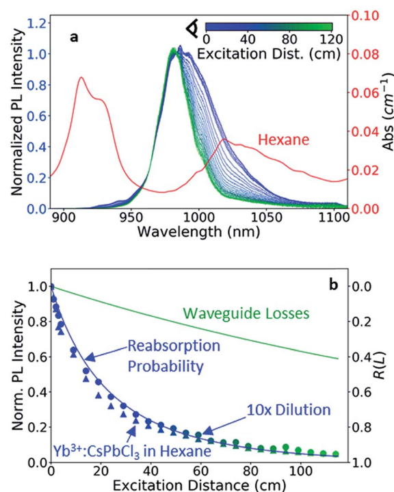
Fig. 2 (a) Normalized PL spectra of \text{Yb}^{3+}:\text{CsPbCl}_3 NCs suspended in hexane with \text{OD}_t \sim 0.75 \text{ mm}^{-1} at 375 nm, obtained from the 1D LSC experiment at various excitation distances relative to the edge-mounted photodetector (see inset). The red curve shows the absorption spectrum of the hexane solvent. (b) Integrated normalized \text{Yb}^{3+}:\text{CsPbCl}_3 NC PL intensity plotted as a function of excitation distance away from the photodetector, for NCs in hexane with \text{OD}_t \sim 0.75 \text{ mm}^{-1} (triangles) and \text{OD}_t \sim 0.075 \text{ mm}^{-1} (circles) at 375 nm. The blue trace is the reabsorption probability described in eqn (1) modeled with hexane absorption from (a). The green line is the experimentally determined performance limit of the 1D LSC. All PL data were collected with excitation at 375 nm, and all data were collected at room temperature.
