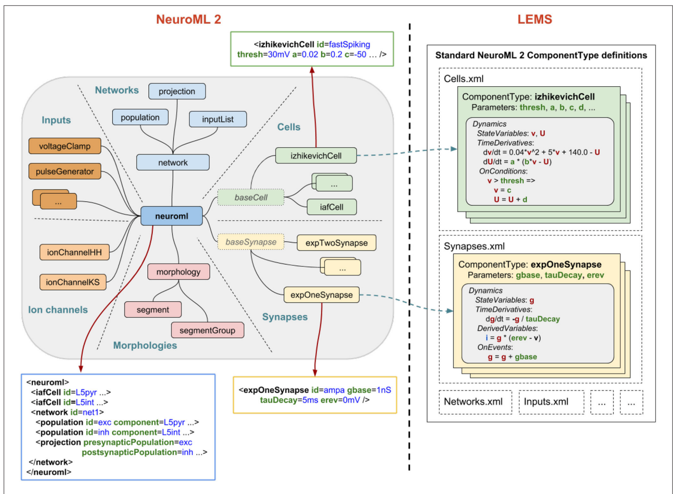
FIGURE 6 | NeuroML2 and LEMS. NeuroML2 is a language which defines a hierarchical set of elements used in computational models in neuroscience in the following broad categories: Networks , Cells , Synapses , Morphologies , Ion Channels , and Inputs . These provide the building blocks for specifying 3D populations of cells, both morphologically detailed and abstract, connected via a variety of (plastic) chemical and electrical synapses receiving external spike or current based stimuli. Examples are shown of the (truncated) XML representations of: (blue) a network containing two populations of integrate-and-fire cells connected by a single projection between them; (green) a spiking neuron model as described by Izhikevich (2003); (yellow) a conductance based synapse with a single exponential decay waveform. On the right the definition of the structure and dynamics of these elements in the LEMS language is shown. Each element has a corresponding ComponentType definition, describing the parameters (as well as their dimensions, not shown) and the dynamics in terms of the state variables, the time derivative of these, any derived variables, and the behavior when certain conditions are met or (spiking) events are received. The standard set of ComponentType definitions for the core NeuroML2 elements are contained in a curated set of files ( Cells.xml , Synapses.xml , etc.) though users are free to define their own ComponentTypes to extend the scope of the language.
