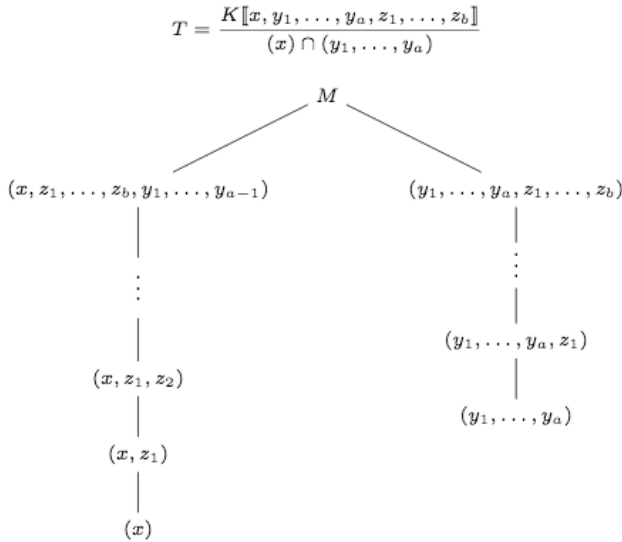
Fig. 2. The Spec diagram for the proof of Proposition 4.1.
