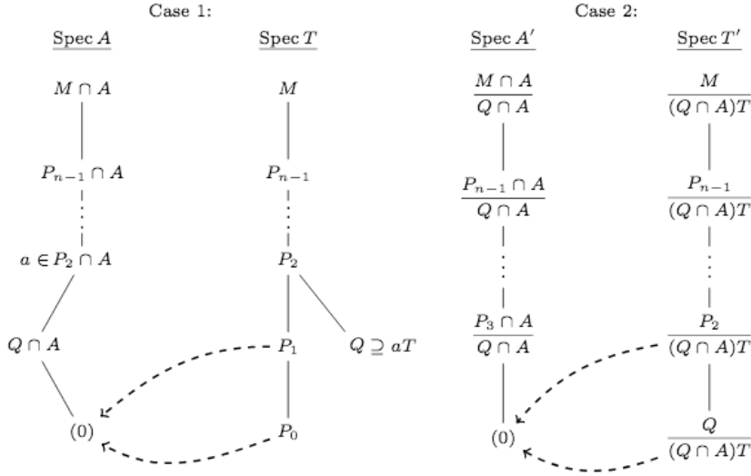
Fig. 1. The Spec diagrams for Case 1 and Case 2 of the proof of Lemma 2.6.
