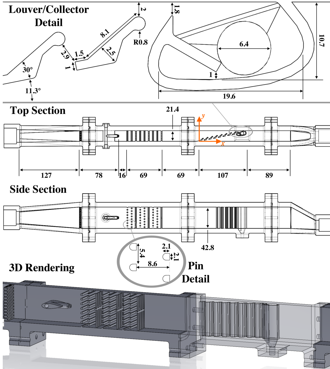
FIGURE 2. SEPARATOR GEOMETRY USED FOR THE PRESENT WORK. FROM BOTTOM TO TOP: 3D RENDERING OF THE FULL GEOMETRY; CUT SECTION VIEWED FROM THE SIDE; CUT SECTION VIEWED FROM THE TOP, WITH COORDINATE ORIGIN SHOWN (ORIGIN IS IN CHANNEL SYMMETRY PLANE); DETAIL VIEW SHOWING COLLECTOR AND LOUVER DESIGN.
