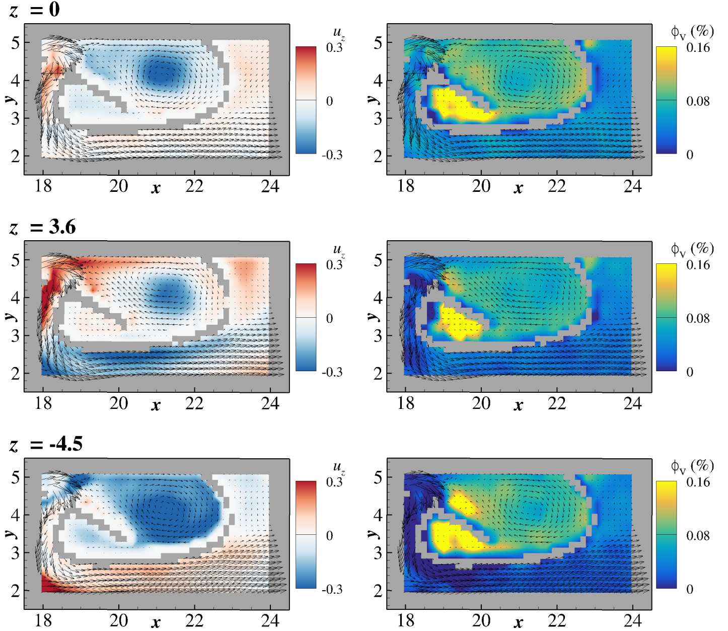
FIGURE 10. DETAIL OF FLOW AND PARTICLE TRANSPORT IN THE COLLECTOR. COLOR CONTOURS OF u_z (LEFT ROW) AND \phi_v (RIGHT) WITH IN-PLANE VELOCITY VECTORS AT THREE SPANWISE LOCATIONS.
