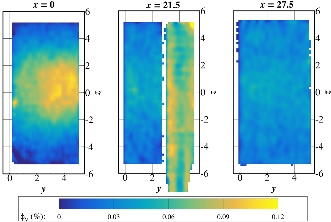
FIGURE 9. Color contours of \phi_V for three planes at x = 0 at the first louver (L), x = 21.5 cutting through the collector (C), and x = 27.5 downstream of the separator (R). Note that the center slice includes the collector wall (white region at y \approx 3 ) and data inside the drain tube protruding below the bottom channel wall at z = -5.5 .
