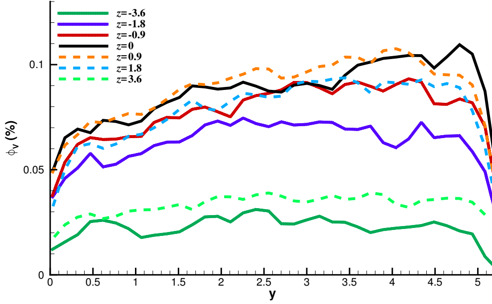
FIGURE 5. WALL-NORMAL ( y ) PROFILES OF \phi_V AT x = -3 . COLOR CORRESPONDS TO ABSOLUTE SPANWISE POSITION, WHILE LINE PATTERN INDICATES +z OR -z SIDE OF CHANNEL.
