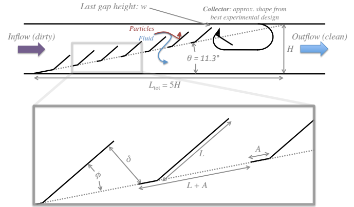
FIGURE 1. DESIGN SPACE FOR LOUVERED PARTICLE SEPARATOR DESIGN OF MUSGROVE ET AL. [5] AND OTHERS.
