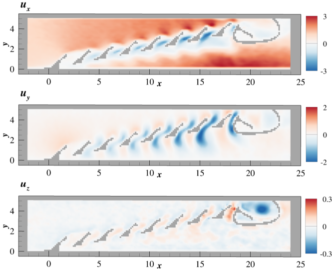
FIGURE 6. COLOR CONTOURS OF u_x (TOP), u_y (CENTER), AND u_z (BOTTOM) IN THE z = 0 PLANE THROUGH THE LOUVERS AND COLLECTOR. ALL VELOCITIES NORMALIZED BY U_{\text{bulk}} = 0.4 m/s.
