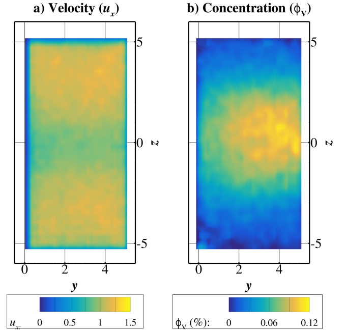
FIGURE 4. COLOR CONTOURS OF STREAMWISE VELOCITY ( u_x ) AND PARTICLE CONCENTRATION ( \phi_v ) FOR THE x = 3 PLANE JUST UPSTREAM OF THE FIRST LOUVER.
