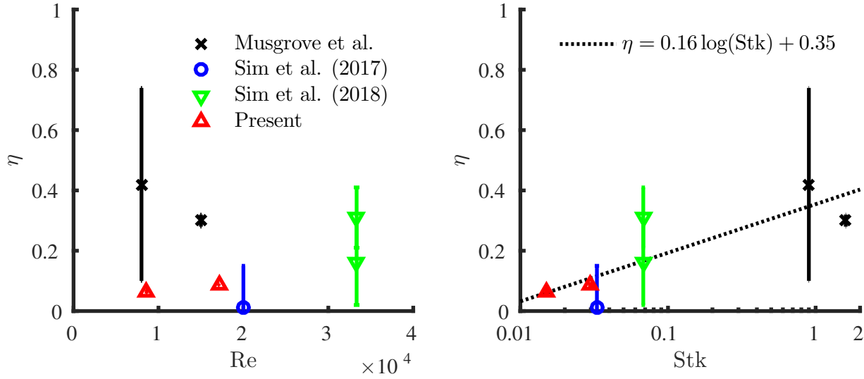
FIGURE 3. SEPARATION EFFICIENCY FOR ALL STUDIES PLOTTED AGAINST REYNOLDS NUMBER (L) AND STOKES NUMBER (R).
