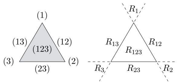
Figure 1. The correspondence between the face-interiors \text{int}(\sigma) that make up the 2-simplex and the regions R_\sigma that deformation retract to the \text{int}(\sigma) ’s (see (3.4)). We define the region R_{12} to contain the face-interior labeled by (12), and R_1 to contain the dashed lines of its boundary and the vertex (1) (so it is closed), which is why in Proposition 3.10 we must pass from the unions of regions R_\sigma to their relative interiors.
