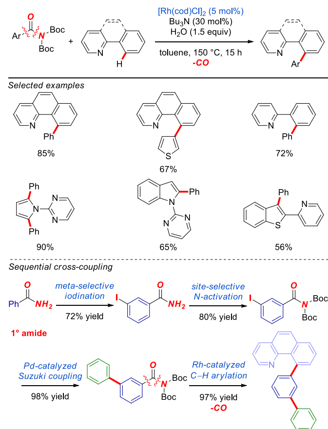
Scheme 8 Rh-catalyzed decarbonylative C–H bond functionalization using N,N-Boc 2 -amides reported our group.
