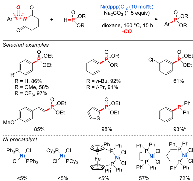
Scheme 11 Ni-catalyzed decarbonylative phosphorylation of amides reported our group. a Using HPPH 2 , 48 h.
