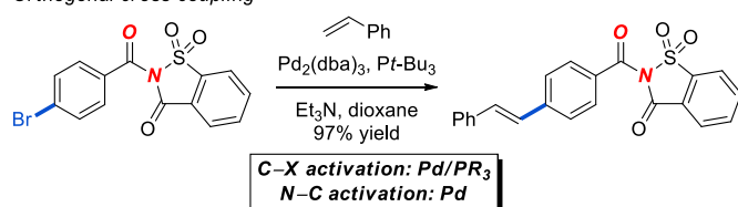
Scheme 2 Pd-catalyzed decarbonylative Heck cross-coupling of N-acyl-saccharins reported by our group.
