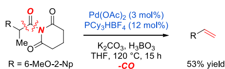
Scheme 6 Pd-catalyzed retro-hydroamidocarbonylation reported by our group.
