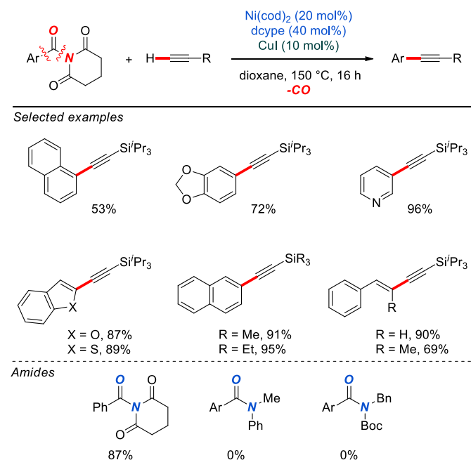
Scheme 18 Ni/Cu-catalyzed decarbonylative alkynylation of amides reported by Rueping and co-workers.
