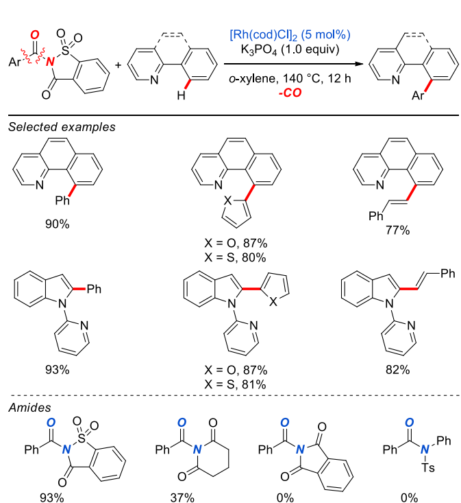
Scheme 9 Rh-catalyzed decarbonylative C–H bond functionalization using amides reported by Zeng and co-workers.
