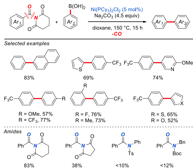
Scheme 10 Ni-catalyzed decarbonylative Suzuki-Miyaura biaryl coupling of amides reported our group.
