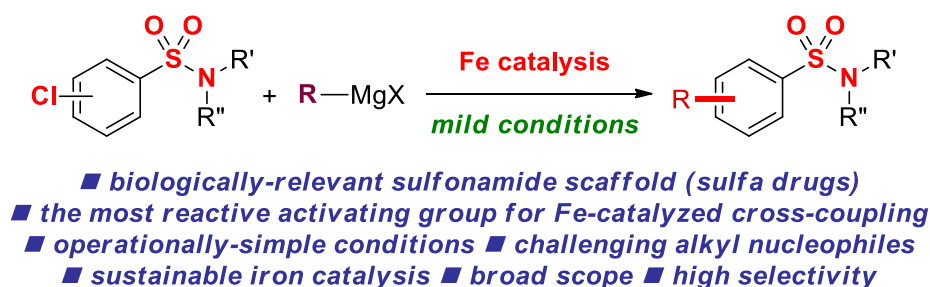
Figure 2. Iron-catalyzed C(sp 2 )-C(sp 3 ) cross-coupling of chloro-benzenesulfonamides with alkyl Grignard reagents (this study).
