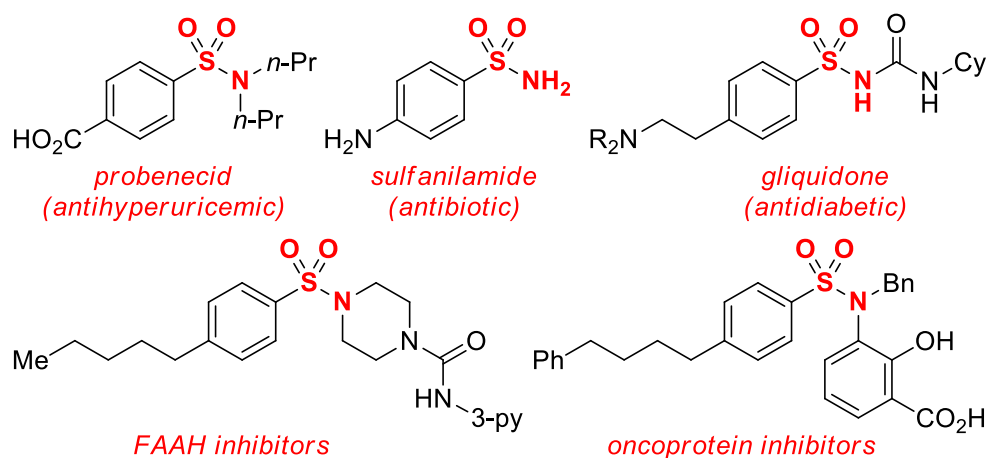
Figure 1. Biologically-active sulfonamides: (a) Classic sulfa drugs (top), and (b) pharmaceutically-active alkylated sulfonamides (bottom).
