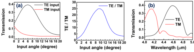
Fig. 4. 2D FDTD simulated transmission for a TE-polarization selective grating coupler versus (a) fiber incident angle and (b) incident wavelength in SoS operating around \lambda=4.55\mu\text{m} .
