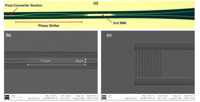
Fig. 7. (a) Microscope image of the polarization rotator. (b) Top view SEM image showing the 2\times 2 multimode interference power splitter section. (c) Top view SEM image of TE selective grating coupler.
