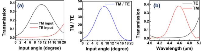
Fig. 5. 2D FDTD simulated transmission for a TM-polarization selective grating coupler versus (a) fiber incident angle and (b) incident wavelength in SoS operating around \lambda=4.55\mu\text{m} .
