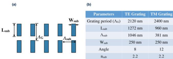
Fig. 6. (a) Schematic illustration of the grating coupler (b) Final design parameters for TE- and TM-polarization selective grating coupler in 900nm thick silicon-on-sapphire. Gratings are broadband.
