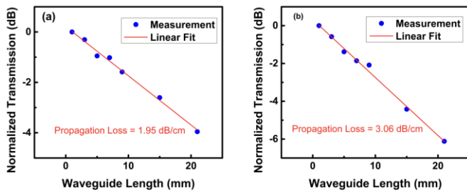
Fig. 8. (a) Propagation loss characteristics of single mode TE strip waveguide in SoS (b) Propagation loss characteristics of single mode TM strip waveguide in SoS
