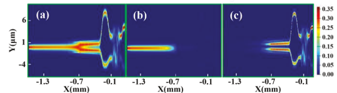
Fig. 3. (a) FDTD simulation showing the electric field intensity magnitude across the complete device with TM_{00} input on the left side and TE_{00} output on the right side. (b) the electric field intensity magnitude of TM components of the propagating wave. (c) the electric field intensity magnitude of TE components of the propagating wave.
