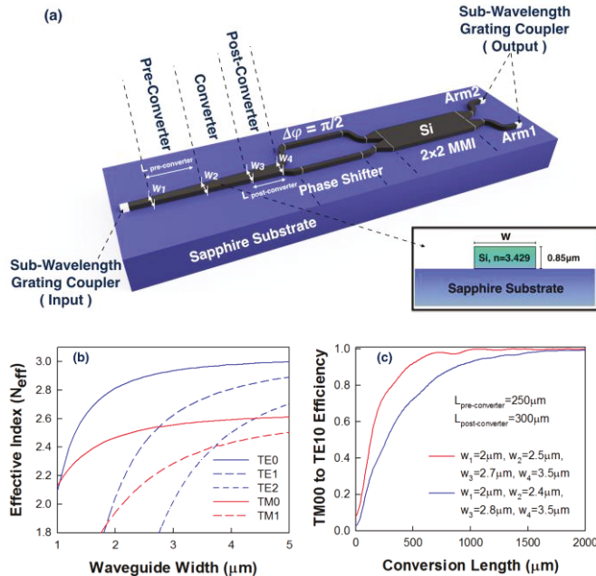
Fig. 1. (a) Schematic of a polarization rotator splitter, similar to the design in Ref. 13. inset is the cross-section geometry of the silicon waveguide, (b) Effective Index versus width ( w ) of waveguide of the propagating waveguide modes simulated by finite-element modeling (FEM) for the waveguide structure in the inset of 1(a), (c) TM_{00} to TE_{10} conversion efficiency at \lambda=4.55\mu m versus length of the converter section for Device1 (red curve) : pre-converter width changes from 2\mu m to 2.5\mu m over 250\mu m , converter width changes from 2.5\mu m to 2.7\mu m and post-converter width changes from 2.7\mu m to 3.5\mu m over 300\mu m and Device2 ( Blue curve) : pre-converter width changes from 2\mu m to 2.4\mu m over 250\mu m , converter width changes from 2.4\mu m to 2.8\mu m and post-converter width changes from 2.8\mu m to 3.5\mu m over 300\mu m .
