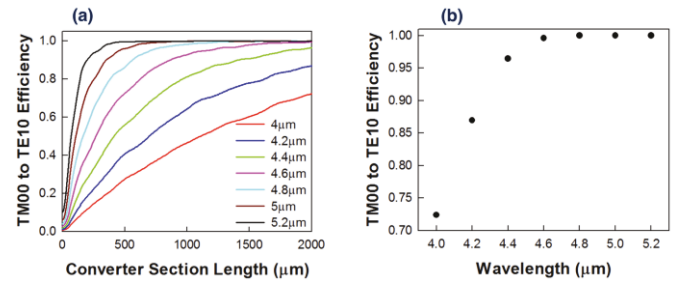
Fig. 2. Eigenmode expansion simulation for conversion efficiency of TM_{00} to TE_{10} as a function of (a) the length of the converter section for different wavelengths and (b) wavelength for 2mm converter length for dimensions given by blue curve in Fig. 1(c).
