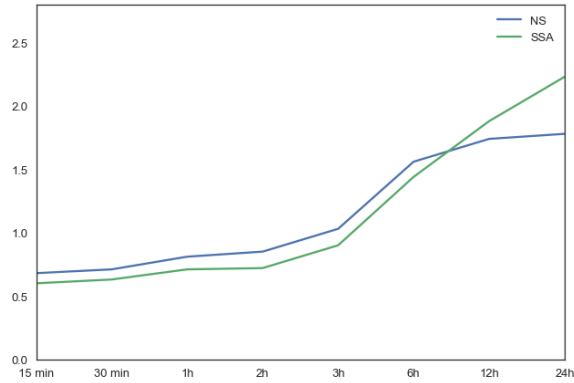
(c) MAE for Goleta-Pi1-WU
