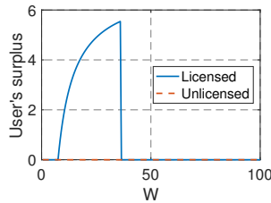
Fig. 5. Variation of users' surplus with W both for licensed and unlicensed spectrum with the same parameters as in Fig. 3.
