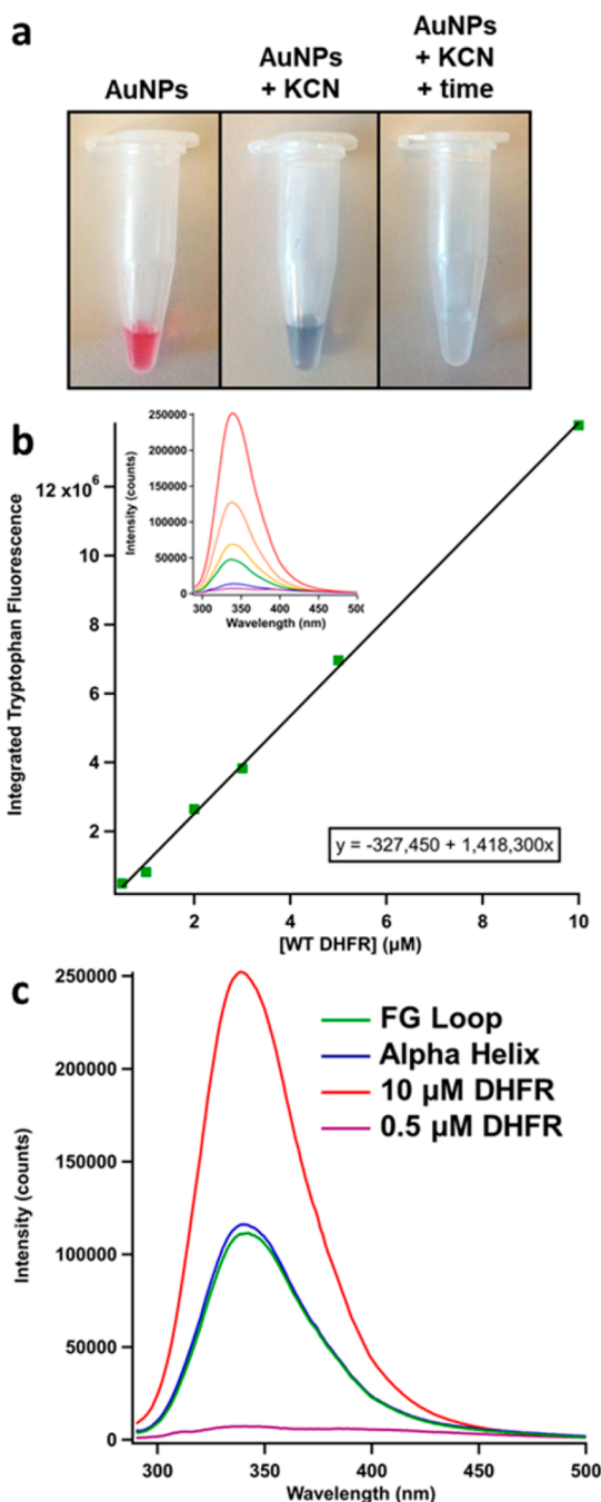
Figure 6. Fluorescence assay for protein concentration determination on the AuNPs. (a) Left: DHFR–AuNP conjugates are stable, as indicated by their pink color. Middle: Immediately after the addition of KCN, the AuNPs start to aggregate, indicated by the deep purple/blue color. Right: After reacting for 1 h, the AuNPs are dissolved and are now Au–KCN complexes, showing no visible color. (b) Standard curve for WT DHFR protein samples under identical conditions as the unknown conjugate samples (same KCN and Tween 20 concentrations). The inset shows the fluorescence spectra obtained with 280 nm excitation. The area under each curve integrated from 300 to 385 nm is plotted versus the respective concentration to form the standard curve. (c) The tryptophan fluorescence spectra for the conjugate samples at the upper and lower bounds of the calibration curve [WT DHFR] and at intermediate concentrations of the mutants (green = FG loop conjugates, blue = alpha helix conjugates). The area under each conjugate spectrum is used in conjunction with the standard curve equation to determine the concentration of protein in the AuNP samples.
