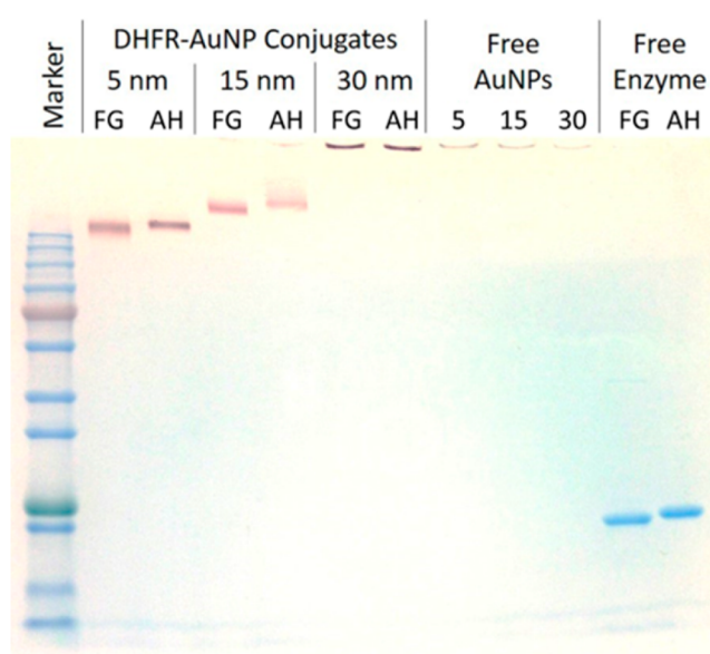
Figure 4. Stained SDS-PAGE gel of DHFR–AuNP conjugates and free DHFR. Lane 1 is protein marker. Lanes 2–3 are 5 nm AuNP–DHFR conjugates. Lanes 4–5 are 15 nm AuNP–DHFR conjugates. Lanes 6–7 are 30 nm AuNP–DHFR conjugates. Lanes 8–10 are free AuNPs: 5, 15, and 30 nm. Lanes 11–12 are free protein. FG = FG Loop mutant. AH = Alpha Helix mutant.
