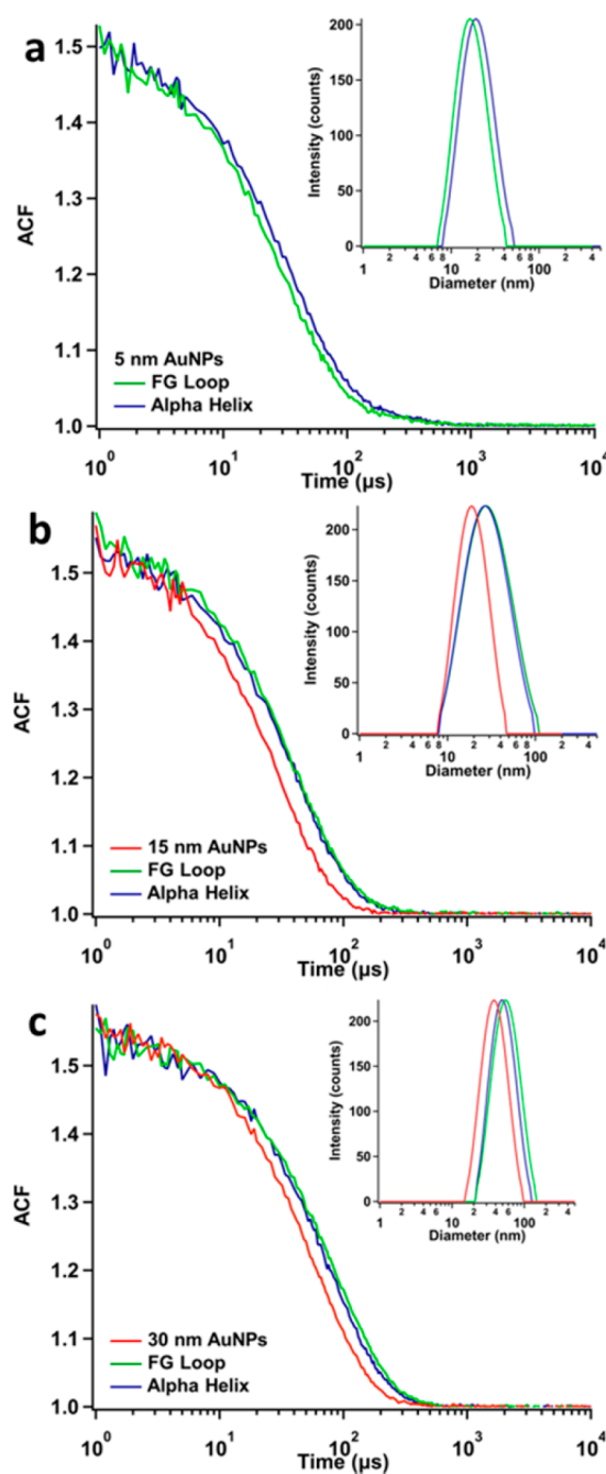
Figure 5. DLS of DHFR–AuNP conjugates. (a) 5 nm AuNP conjugates: (green) FG loop conjugates (16.5 nm), (blue) Alpha Helix conjugates (19.4 nm). Free AuNPs are too small to obtain accurate DLS measurements. (b) 15 nm AuNP conjugates: (red) free 15 nm AuNPs (18 nm), both AuNP–DHFR conjugates (27 nm). (c) 30 nm AuNP conjugates: free 30 nm AuNPs (35 nm), FG loop conjugates (48 nm), Alpha Helix conjugates (46 nm).
