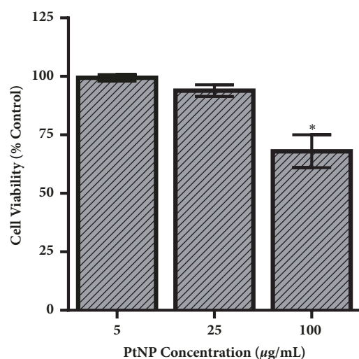
FIGURE 2: HepG2 viability following PtNP exposure. HepG2 liver cells underwent a 24-hour exposure to PtNPs at varying dosages, followed by evaluation of cellular viability. At the highest PtNP dosage, a significant toxicity response was observed. Data represents 3 independent trials with * denoting statistical significance from untreated controls ( p < 0.05 ).
