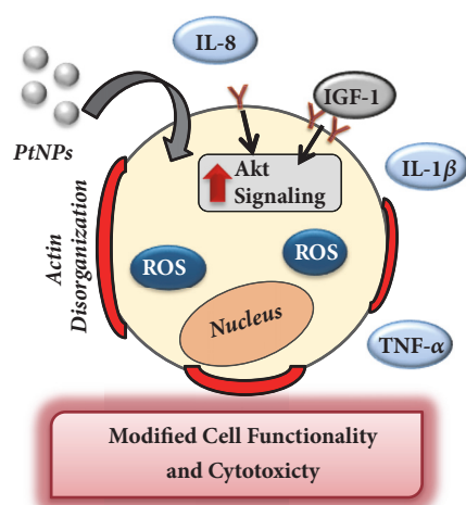
FIGURE 6: Summary of HepG2 cellular responses following PtNP exposure. This study identified that PtNPs induced traditional toxicological responses including cytotoxicity and stress activation. Moreover, cellular functionality was modified as assessed via activation of an inflammatory response and modulation of IGF-1 dependent signal transduction.
