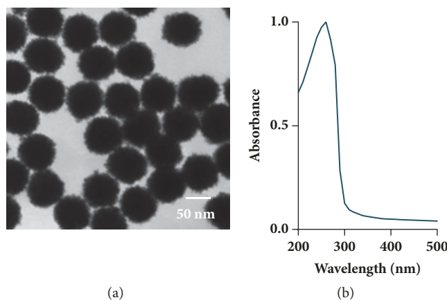
FIGURE 1: Characterization of the experimental PtNPs. (a) A representative TEM image of the experimental PtNPs was used to verify primary size and morphology. (b) The PtNP stock underwent UV-Vis analysis in order to obtain the unique spectral signature for these particles.
