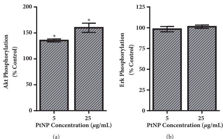
FIGURE 5: Evaluation of IGF-1 dependent signal transduction. HepG2 cells were exposed to PtNPs and then stimulated with IGF-1 to induce the PI3K/Akt and Ras/Erk signaling pathways. Activation of these cascades was assessed via normalized phosphorylation levels of (a) Akt and (b) Erk, respectively. Data represents 3 independent trials with * denoting statistical significance from untreated controls ( p < 0.05 ).
