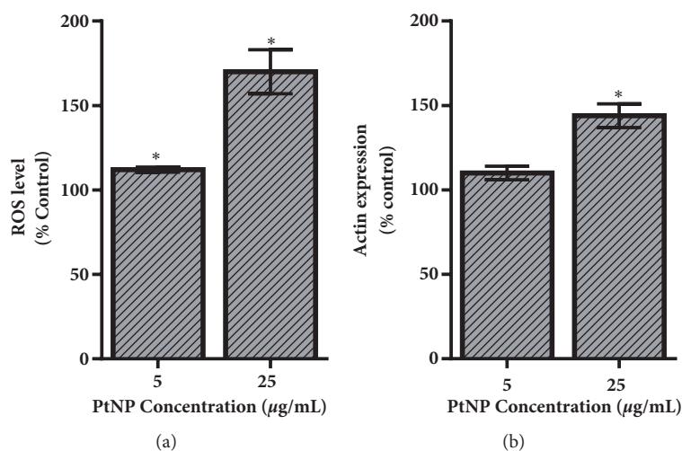
FIGURE 3: PtNP-induced stress response within the HepG2 cell model. (a) ROS and (b) actin levels were measured within HepG2 cells following a 24-hour exposure to varying dosages of PtNPs. Both endpoints demonstrated a dose-dependent increase in stress activation. Data represents 3 independent trials with * denoting statistical significance from untreated controls ( p < 0.05 ).
