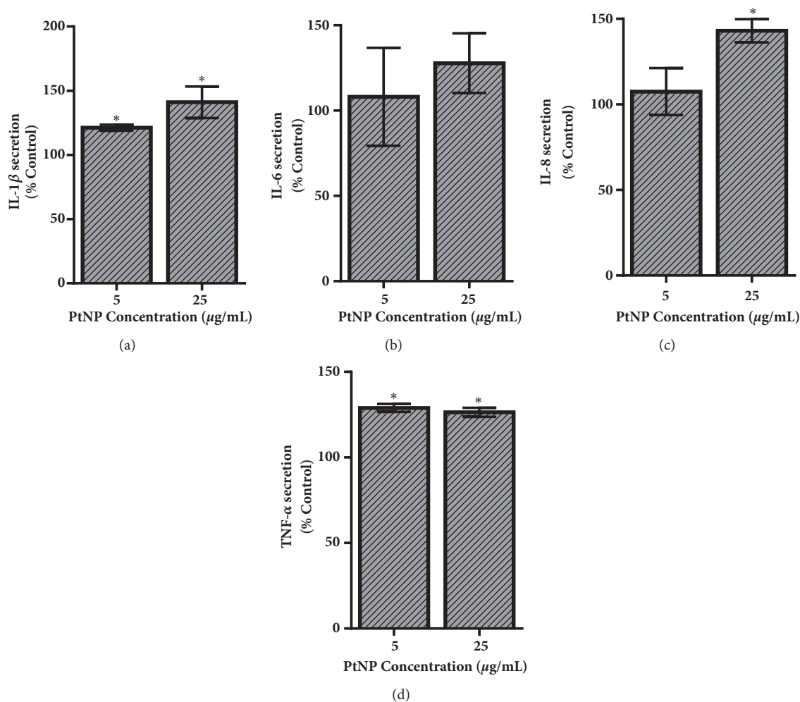
FIGURE 4: Activation of the HepG2 inflammatory response. To assess PtNP-dependent inflammatory activation, secretion levels of key proinflammatory cytokines were quantified. Following a 24-hour exposure to varying levels of PtNPs, the media were recovered from the HepG2 culture and underwent analysis for (a) IL-1 \beta , (b) IL-6, (c) IL-8, and (d) TNF- \alpha . Data represents 3 independent trials with * denoting statistical significance from untreated controls ( p < 0.05 ).
