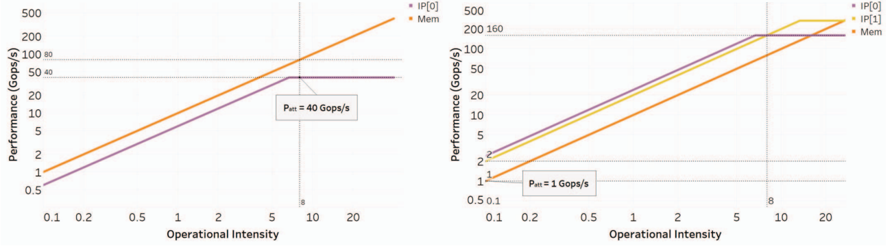
(a) With initial parameters, performance matches CPU's 40 Gops/s at assumed operational intensity I_0 = 8 , as the GPU is not used.
