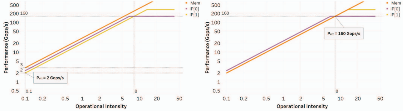
(c) Increasing memory bandwidth B_{peak} from 10 to 30 GB/s increases performance to only 2 Gops/s.
