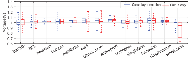
Fig. 11. Noise distribution across benchmarks and the worst-case imbalance.
