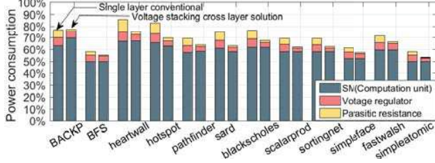
Fig. 16. Applying PG on conventional and proposed voltage-stacked GPU.
