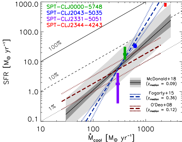
FIG. 8.— BCG star formation rate compared to classical cooling rate ( \dot{M}_{cool} \equiv \dot{M}_g(r < r_{cool})/t_{cool} ) for the four clusters in our sample. These star formation rates are based on the [O II] emission line, and are corrected for intrinsic extinction as measured from the CIGALE fit to the broadband SED. For comparison, we show the relations found in O’Dea et al. (2008, dark red) and McDonald et al. (2018, black/grey) for clusters at z \sim 0.1 . For the latter, we show the uncertainty on the fit in dark grey, and the measured scatter in light grey. In blue, we show the fit to CLASH clusters from Fogarty et al. (2015), which are at considerably higher redshift. Overall, the relaxed clusters in the SPT sample (including Phoenix, (McDonald et al. 2012), which is the most relaxed SPT-selected cluster) tend to host BCGs with higher SFR per unit cooling ICM than clusters at z \sim 0 .
