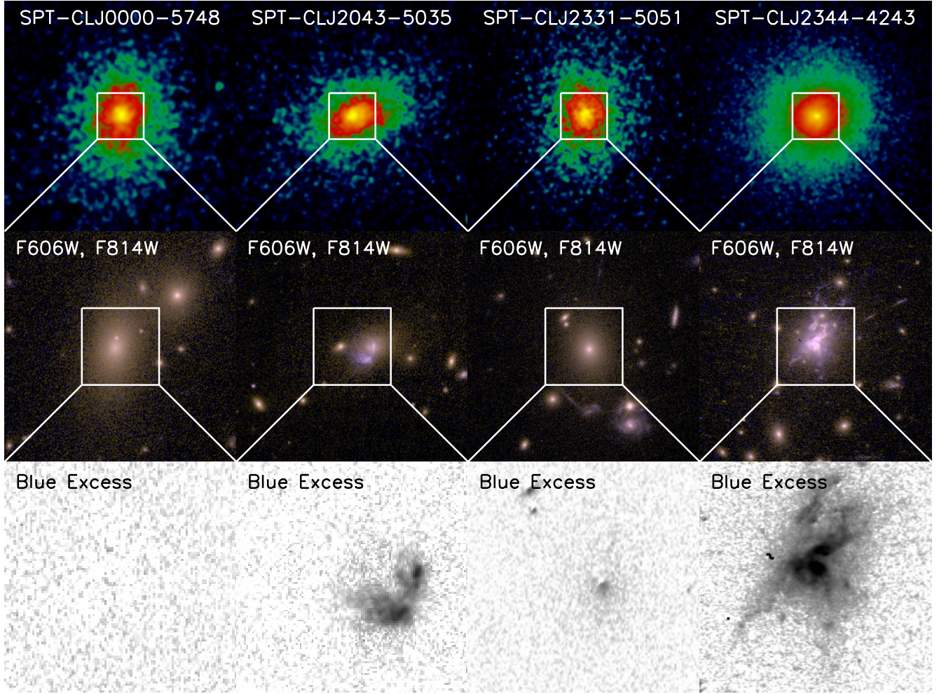
FIG. 7.— Upper row : X-ray image (0.7–4.0 keV) of each cluster, showing the relatively relaxed, centrally-concentrated morphology. Images are 1 Mpc on a side. Middle row : Zoomed-in optical images of the cluster core, showing the central BCG in each cluster. These images are made by combining the F606W (blue) and F814W (green, red) images from HST in such a way as to make the old stellar populations appear red and the young populations blue. Both SPT-CLJ0000-5748 and SPT-CLJ2331-5051 appear relatively quiescent in these colors, while SPT-CLJ2043-5035 and SPT-CLJ2344-4243 clearly have significant younger stellar components. Lower row : Zoomed in image showing the excess emission in the F606W band above the expectation for a passive stellar population, based on the F814W band image. These panels show an absence of emission for the quiescent (based on color) BCGs, and clumpy, extended emission for SPT-CLJ2043-5051 and SPT-CLJ2344-4243. This clumpy, blue emission, which is extended on scales of \sim 15 kpc (SPT-CLJ2043-5051) and \gtrsim 50 kpc (SPT-CLJ2344-4243), is further evidence for ongoing star formation.
