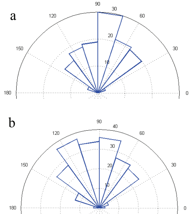
Fig. 5. Rose diagrams of opening-mode microcrack orientation for synthetic salt-rock with (a) axial strain = 2.4%; (b) axial strain = 4.3%; the angle is between the major axis of the best fit ellipse of the microcrack and the direction perpendicular to load axis (90° is in the direction of axial stress).
