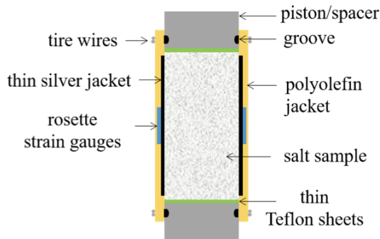
Fig. 1. Schematic of sample instrumentation for cyclic triaxial compression tests
