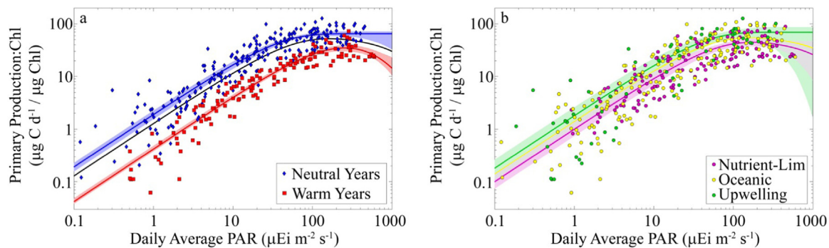
Fig. 3. Functional relationship of phytoplankton production to light. a) Warm vs. neutral years. Functional relationship is: PP/chl = V_{0m} \times [1 - \exp(-\alpha PAR/V_{0m})] \times \exp(-\beta PAR/V_{0m}) . Black line shows the relationship for all data, red and blue lines for warm and neutral years, respectively. b) As in (a) except data are grouped by water parcel type (nutrient-limited, transition region, coastal upwelling). Error bounds show 95% confidence intervals for the functional relationship (not for prediction of individual points) as determined by non-parametric bootstrapping uncertainty analysis. Error bounds are not shown for transition region data in (b). (For interpretation of the references to color in this figure legend, the reader is referred to the web version of this article.)
