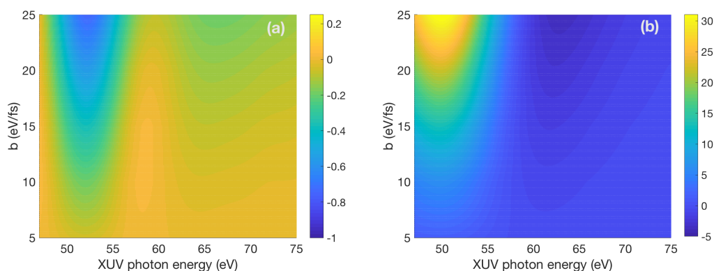
Figure 6. Difference between streaking time delays \Delta t_s(b) - \Delta t_s(b=0) (in attoseconds) in a chirped to those in an unchirped pulse for photoemission from (a) 2p shell of neon atom and (b) 3p shell of argon atom as function of electron energy and chirp parameter.
