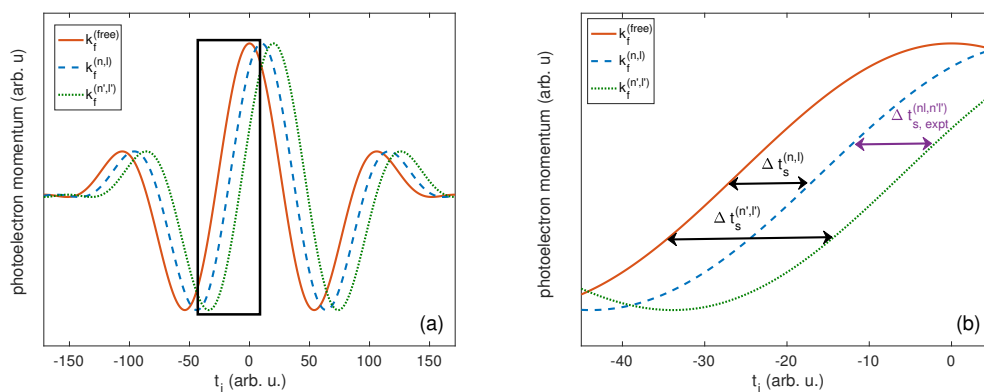
Figure 1. Conceptual visualization of the different streaking time delays in photoionization, namely the experimentally observed delay \Delta t_{s,expt}^{(nl,n'l')} between streaking traces for emission from initial states |n,l\rangle and |n',l'\rangle and the theoretically considered delays \Delta t_s^{(nl)} and \Delta t_s^{(n'l')} with respect to the streaking trace of a free electron. Panel (b) is an enlargement of the full traces shown in panel (a).
