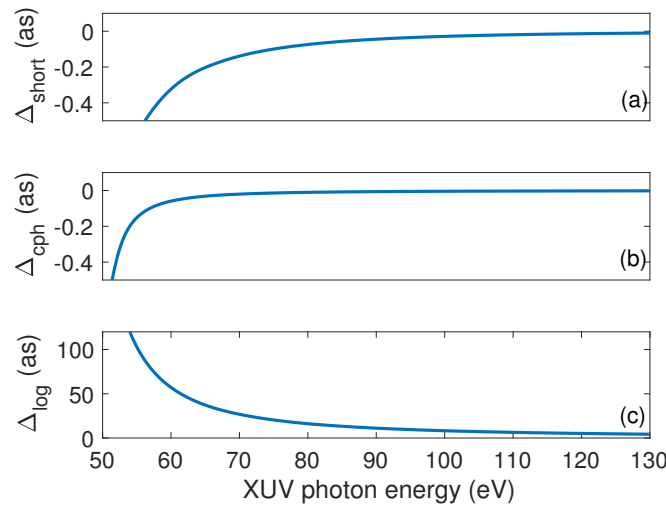
Figure 4. Absolute difference for the different contributions to the time delay of neon atom with and without the effect of the streaking field as a function of electron energy and streaking field wavelength: (a) short-range contribution; (b) Coulomb phase contribution; and (c) Coulomb logarithmic contribution. Parameters of the streaking field: wavelength \lambda_s = 800 nm, peak intensity I_s = 1 \times 10^{12} W/cm 2 , and pulse duration of three cycles is used [23].
