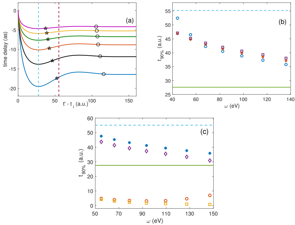
Figure 5. (a) Analytical predictions for the streaking time delay (in attoseconds) of hydrogen atom as a function of time t' - t_i (in atomic units) for electron kinetic energies corresponding to XUV central frequencies of \omega = 44.22 eV (blue), \omega = 55.27 eV (black), \omega = 68.03 eV (red), \omega = 82.48 eV (green), \omega = 98.64 eV (yellow), and \omega = 116.49 eV (pink) and a three-cycle streaking pulse. The times t_{90\%} and t_{99\%} are shown as stars and circles, respectively, and T/4 and T/2 are denoted with dashed vertical lines; (b) time t_{90\%} (in atomic units) is shown as a function of XUV central frequency for different streaking pulse durations; N_s = 3 cycles (circles), N_s = 4 cycles (stars), N_s = 5 cycles (diamonds), and N_s = 6 cycles (squares). Further shown is T/2 (dashed light blue) and T/4 (solid green); (c) same as panel (b) but for helium atom and the separate contributions, short-range (circles), Coulomb-phase (squares), logarithmic (diamonds), and the total (stars) in a three-cycle streaking pulse. For all calculations, a streaking pulse of wavelength \lambda_s = 800 nm and I_s = 1 \times 10^{12} W/cm 2 has been considered.
