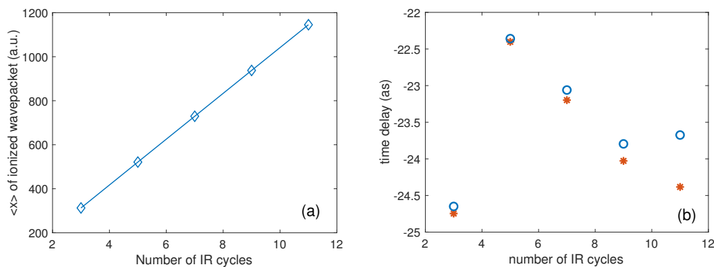
Figure 3. (a) Range of wavepacket propagation in an 800 nm streaking pulse after emission at the peak of the pulse as a function of the number of cycles for 1D soft-core model; (b) streaking time delay in a potential with additional perturbation (stars) at x_0 = 850 a.u. as compared to the delay obtained without the additional potential (circles) as a function of the number of cycles.
