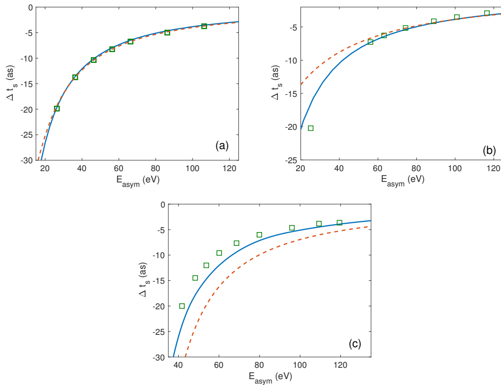
Figure 2. Streaking time delays for hydrogen atom (a); helium atom (b); and neon atom (c): a comparison of results of ab initio calculations is shown (open squares, taken from [24] for hydrogen and helium, [25] for neon), classical calculations (solid lines, Equation (8)) and predictions of analytical model formula (dashed lines, Equation (11)). For neon atoms, only the d-channel is considered in the analytical calculation.
