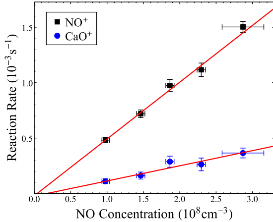
FIG. 4. Measured reaction rates for product channels \text{NO}^+ and \text{CaO}^+ as a function of the neutral NO concentration in the chamber. The NO pressure in the chamber was varied between 3.4 \times 10^{-9} and 1 \times 10^{-8} Torr to change the NO concentration. For all of these data, the P_{1/2} -state population was 19.1% (1.8%). The slopes of the fit lines correspond to the 180 K reaction rate constants.
