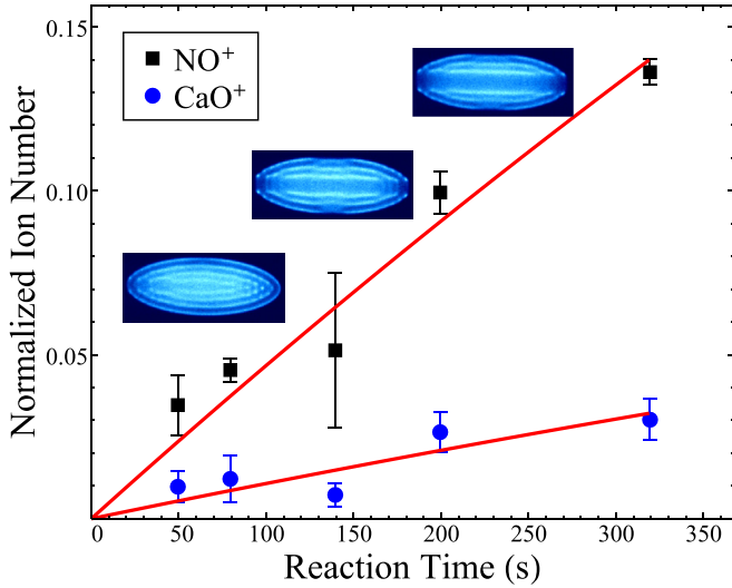
FIG. 2. \text{NO}^+ and \text{CaO}^+ measured ion numbers as a function of time. Ion numbers are normalized by the initial number of \text{Ca}^+ determined from the image captured at t = 0 . Error bars represent the standard error of the mean of measured ion numbers from five experimental runs at each time point. Solid lines indicate fits to the data using a pseudo-first-order reaction rate model. Also shown are three false-color fluorescence images of the Coulomb crystals taken immediately before ejecting the ions into the TOFMS. Images were taken at t = 50, 200 , and 320 s. Dark bands in the center and along the outer edges of the crystals indicate the presence of ions that are lighter and heavier than \text{Ca}^+ , respectively. These ions are the reaction products.
