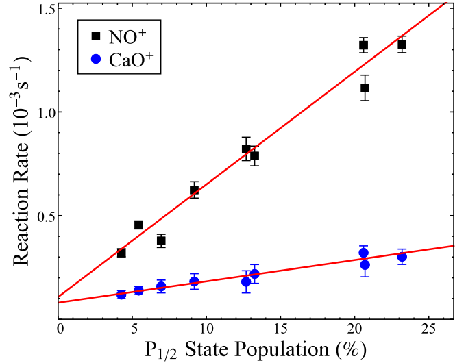
FIG. 3. Measured reaction rates for the two product channels, \text{NO}^+ and \text{CaO}^+ , as a function of the \text{Ca}^+ P_{1/2} -state population. The NO concentration was 2.3(1) \times 10^8 \text{ cm}^{-3} for all of these data. The initial number of \text{Ca}^+ ions in the trap was around 600. The slopes of the fit lines are used to determine the 180 K reaction rate constants. The statistical uncertainty in the P_{1/2} -state population is smaller than the symbols. There is an offset for the reaction rate at zero excited-state population. However, it corresponds to only a 1%–2% offset in the P_{1/2} -state population, which is likely due to a small systematic in determining the absolute state population from the fluorescence.
