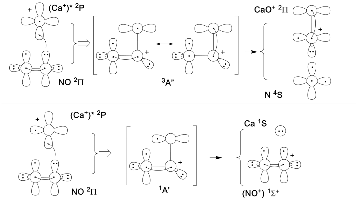
FIG. 5. Top: Generalized valence-bond diagrams that illustrate the processes whereby ^2P calcium atoms react with NO molecules to form \text{CaO}^+ and nitrogen atoms in their ground states. Bottom: Charge exchange process that yields Ca atoms and ground-state \text{NO}^+ .
