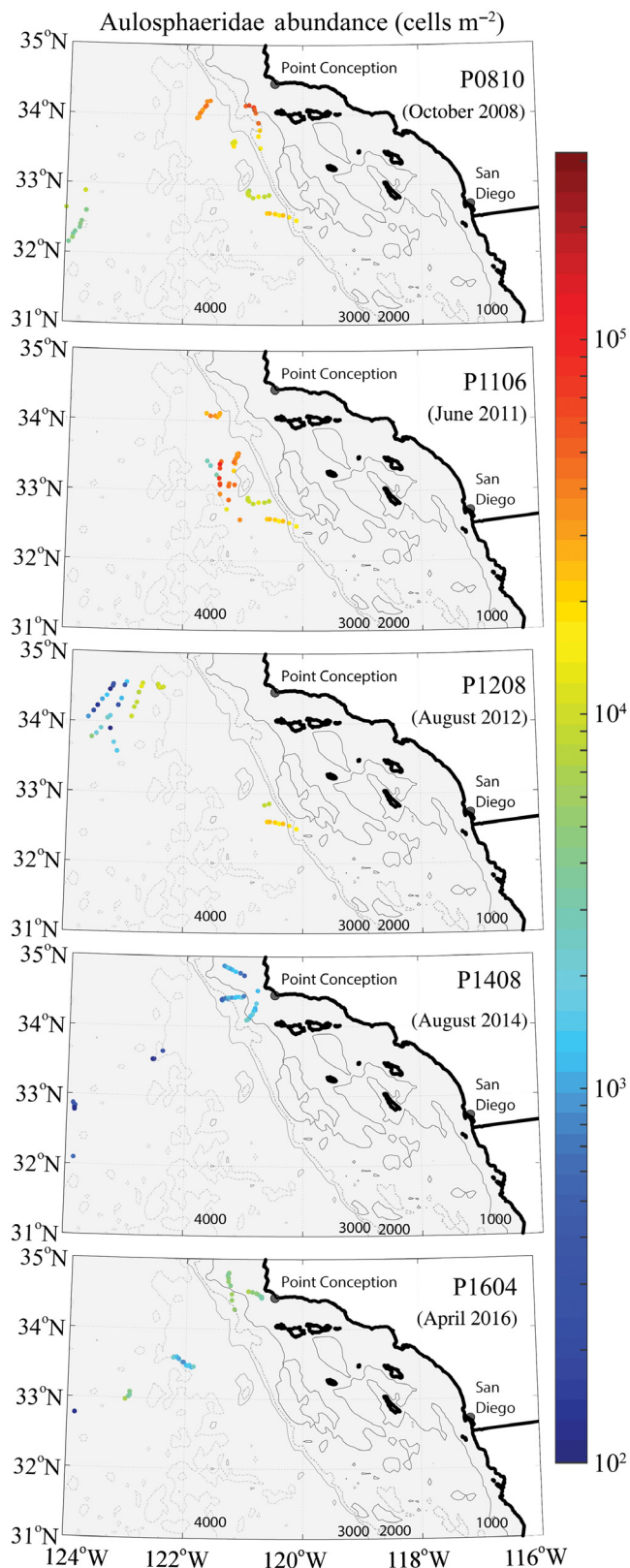
Fig. 1. Aulosphaeridae vertically integrated abundance (cells m -2 ) measured by UVP5 on individual CTD casts on each of our cruises. Contour lines are bathymetry (m).
