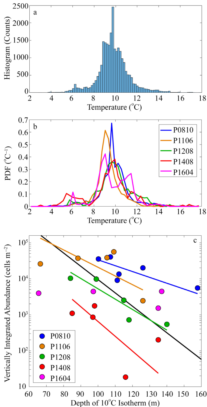
Fig. 4. Histogram of temperatures for each Aulosphaeridae encountered (a). Probability density function for temperatures of Aulosphaeridae for each individual cruise (b). Aulosphaeridae abundance plotted against the depth of the 10°C isotherm (c). Black regression line is a Type II geometric mean regression of \log_{10}(\text{abundance}) against depth. Correlation coefficient is -0.31 . Colored lines are regressions for individual years. Correlation coefficients are -0.75 (2008), -0.52 (2011), -0.93 (2012), and -0.65 (2014).
