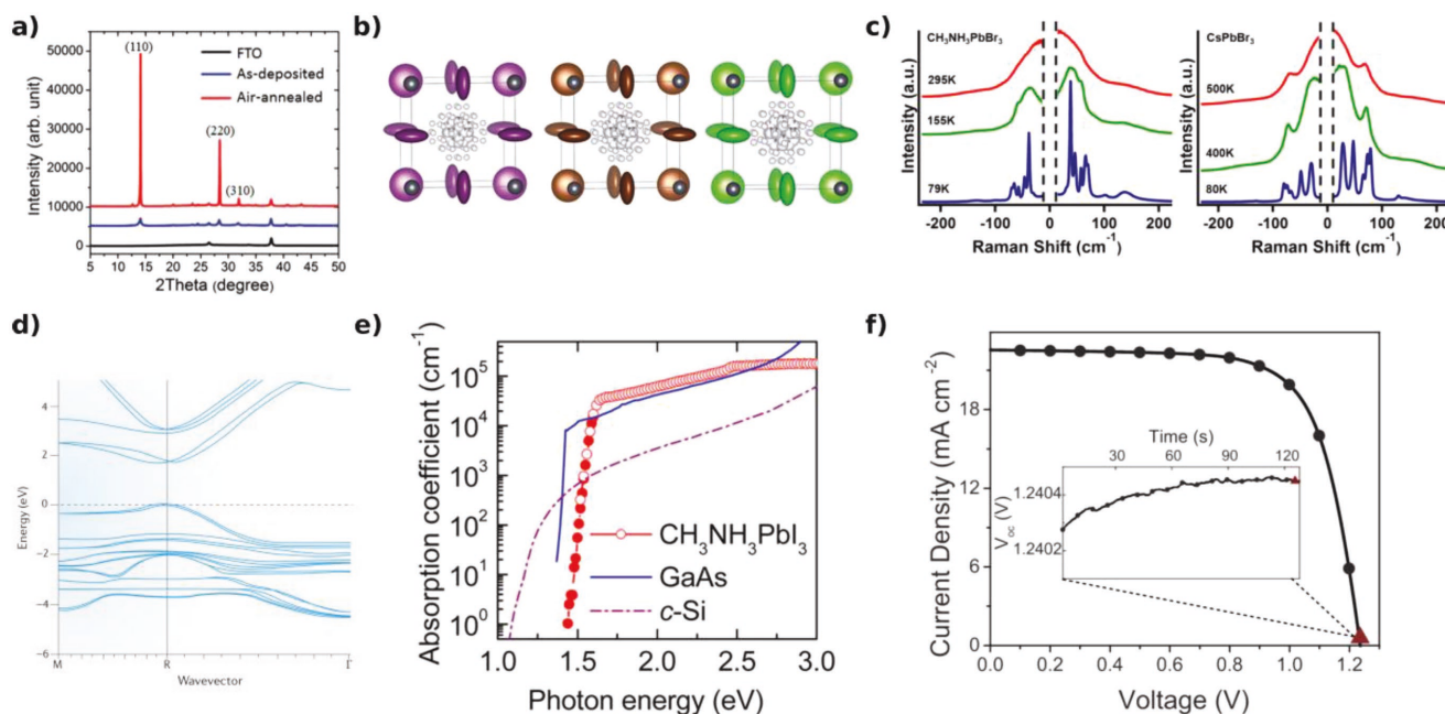
Figure 1. Halide perovskites (HaPs) exhibit a unique combination of structural and optoelectronic properties: a–c) the upper part shows selected data associated with the former, and d–f) the lower part the same for the latter. a) X-ray diffraction (XRD) spectra of as-deposited and air-annealed MAPbI 3 films (annealing was performed at 150 °C for 15 min). b) Refined structures of MAPbX 3 single crystals (with X being I, Br, and Cl, from left to right) obtained from XRD and neutron diffraction experiments showing the disordered arrangement of the MA groups and large displacement ellipsoids of the halides. c) Low-frequency Raman spectra of hybrid and inorganic HaPs in the orthorhombic (blue), tetragonal (green), and cubic phase (red), showing growth of the central peak with temperature in both materials. d) Electronic band structure of cubic-phase MAPbI 3 calculated with many-body perturbation theory in the GW approximation. M, R, and Γ correspond to (1/2, 1/2, 0), (1/2, 1/2, 1/2) and (0, 0, 0) k-points, respectively. e) Effective absorption coefficient of a MAPbI 3 thin film compared with GaAs and crystalline silicon (c-Si), all measured at room temperature. f) Current–voltage curve of high open-circuit voltage (V oc ) device made with a (Rb, Cs, MA, FA) HaP alloy as the absorber material (optical gap: 1.63 eV). The inset shows the V oc as function of time resulting in 1240 mV, which is displayed as the red triangles in both plots. a) Reproduced with permission. [9] Copyright 2015, Wiley-VCH. b) Reproduced with permission. [25] Copyright 2015, Royal Society of Chemistry. Panel (c) reprinted with permission. [15] Copyright 2017, American Physical Society. d) Reproduced with permission [5] (data originally reported in ref. [28]) Copyright 2016, Nature Publishing Group. e) Reproduced with permission. [31] Copyright 2014, American Chemical Society. f) Reproduced with permission. [61] Copyright 2016, American Association for the Advancement of Science.
