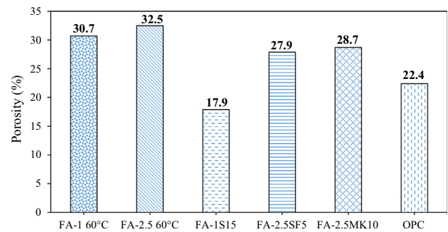
Fig. 9. Porosity of AAFA and OPC pastes.
