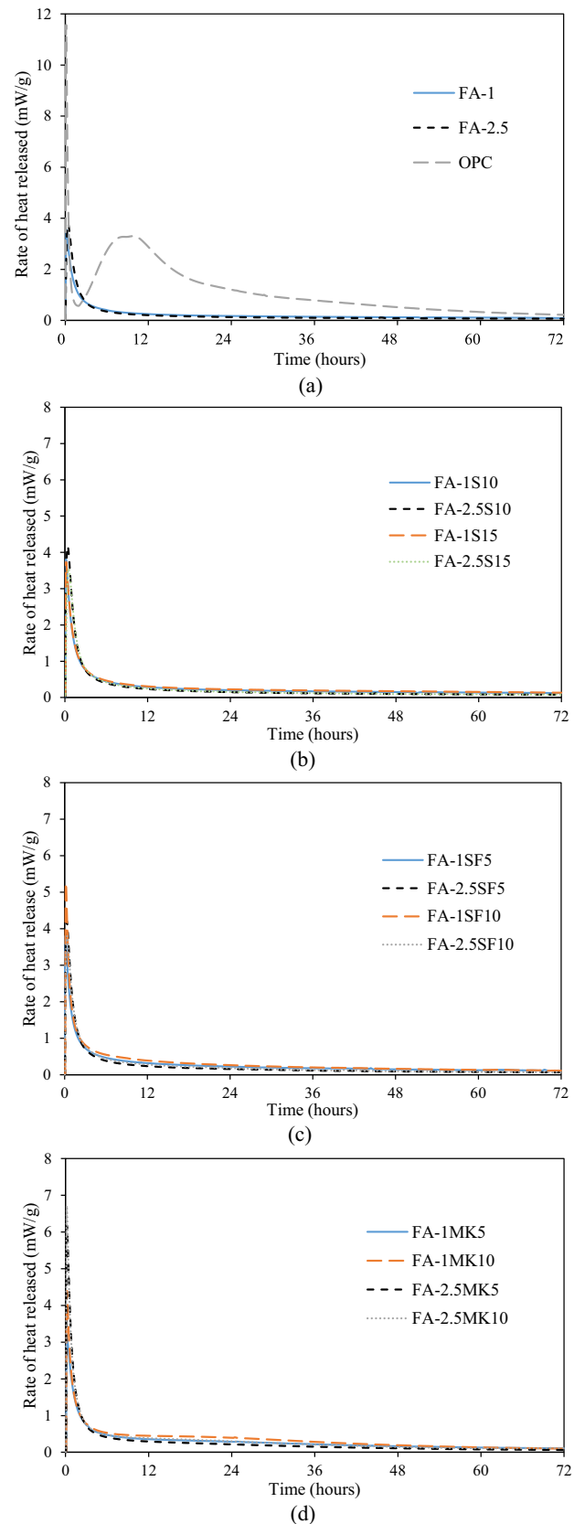
Fig. 2. Heat evolution comparison. (a) Reference mixes, (b) Effect of slag and SS/SH, (c) Effect of silica fume and SS/SH, and (d) Effect of metakaolin and SS/SH.
