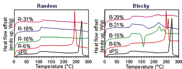
Fig. 4 DSC heating scans of the sPS homopolymer and the (left) Random and (right) Blocky copolymers after rapid cooling from the melt (300 °C) at -60\text{ °C min}^{-1} . Heating rate: 10\text{ °C min}^{-1} .
