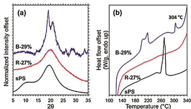
Fig. 7 (a) Wide-angle X-ray diffraction profiles of the melt-quenched Blocky B-29%, Random R-27%, and the sPS homopolymer samples, and (b) DSC heating scans of the Blocky B-29%, Random R-27%, and the sPS homopolymer samples following 1 h isothermal crystallization at 190 °C.
