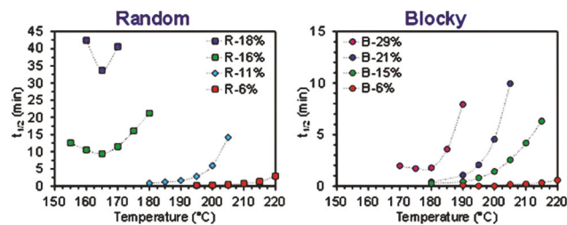
Fig. 5 Crystallization half-time ( t_{1/2} ) versus temperature profiles for the (left) Random and (right) Blocky copolymers. The t_{1/2} scales are different to clearly demonstrate the rapid crystallization kinetics, small t_{1/2} times, exhibited by the Blocky samples.
