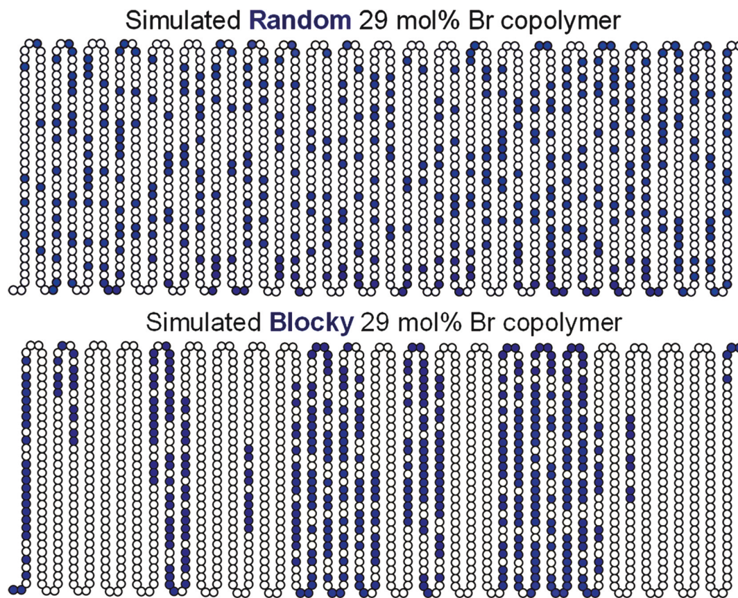
Fig. 9 Representative 29 mol% Br (top) random and (bottom) blocky copolymer chains derived from simulations. Each comonomer sequence is 1 of the 1000 copolymer chains of 1442 monomer units generated in the simulations. The particular sequence selected has a prevalence of pure styrene pentads (SSSSS, where S = styrene) that is most similar to the average number of SSSSS for all 1000 simulated chains. Open circles = styrene; filled circles = Br-Sty.
