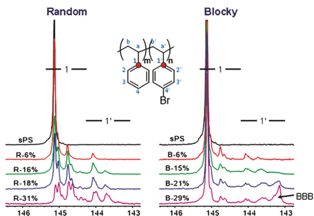
Fig. 3 C(1) and C(1') NMR spectra of the (left) Random and (right) Blocky copolymers increasing in mol% Br from top to bottom. For comparison, spectra are referenced to TCE-d 2 and normalized over 127.0–132.5 ppm.
