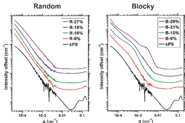
Fig. 6 USAXS/SAXS profiles of quenched films of the sPS homopolymer and the (left) Random and (right) Blocky copolymers. Films were prepared from powders of the homopolymer or copolymers by melt pressing between Kapton sheets at 30 °C above T_m for 20 s at 2200 psi then for 20 s at 4500 psi, followed by quenching in ice water to prevent sPS crystallization. For clarity, the scattering profiles and vertically offset.
