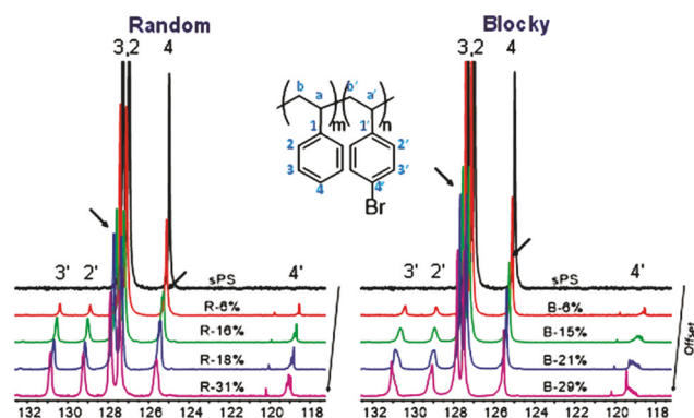
Fig. 2 Aromatic \text{C}(\text{2}-\text{4}) and \text{C}(\text{2}'-\text{4}') resonances in the ^{13}\text{C} NMR spectra of the (left) Random and (right) Blocky copolymers increasing in mol% Br from top to bottom. For comparison, spectra are referenced to \text{TCE}-\text{d}_2 and normalized over 127.0–132.5 ppm.
