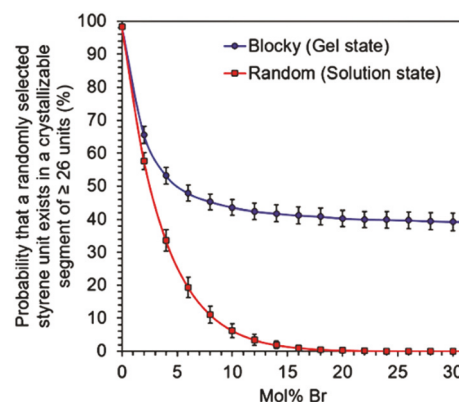
Fig. 8 Probability that a styrene unit selected at random exists in a crystallizable segment of at least 26 consecutive styrene units from simulations of theoretical blocky (gel-state) or random (solution-state) copolymers. Results based on 1000 polymer chains of 1442 monomer units. Error bars represent one standard deviation.
