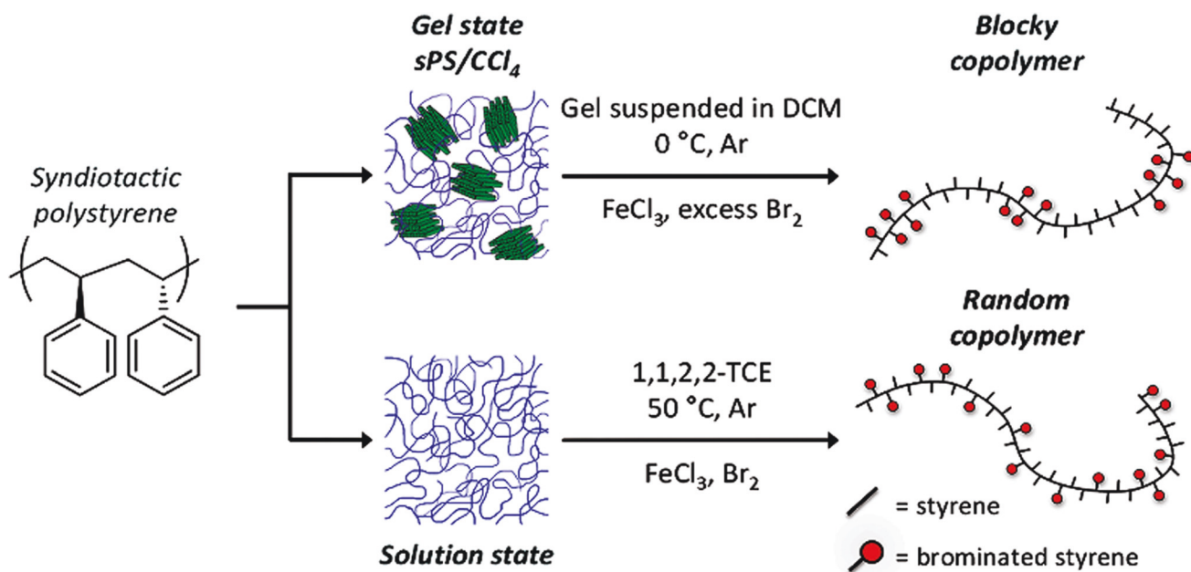
Scheme 1 Schematic representation of sPS bromination via post-polymerization functionalization in solution and in the heterogeneous gel state.
