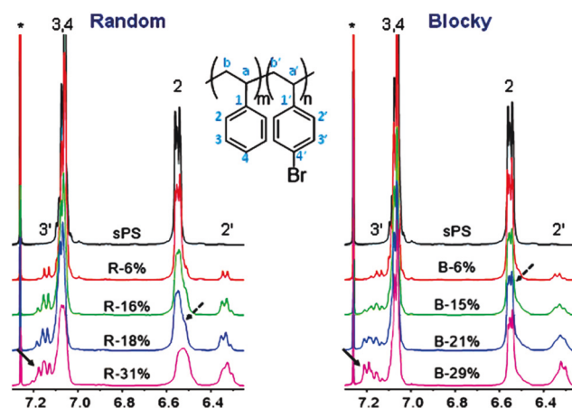
Fig. 1 Aromatic region of the ^1\text{H} NMR spectra of (left) solution-state Random and (right) gel-state Blocky copolymers increasing in mol% Br from top to bottom. For comparison, spectra are referenced to \text{CDCl}_3 and normalized over 6.27–6.60 ppm. The asterisk (*) indicates solvent resonance. The arrows highlight differences between spectra.
