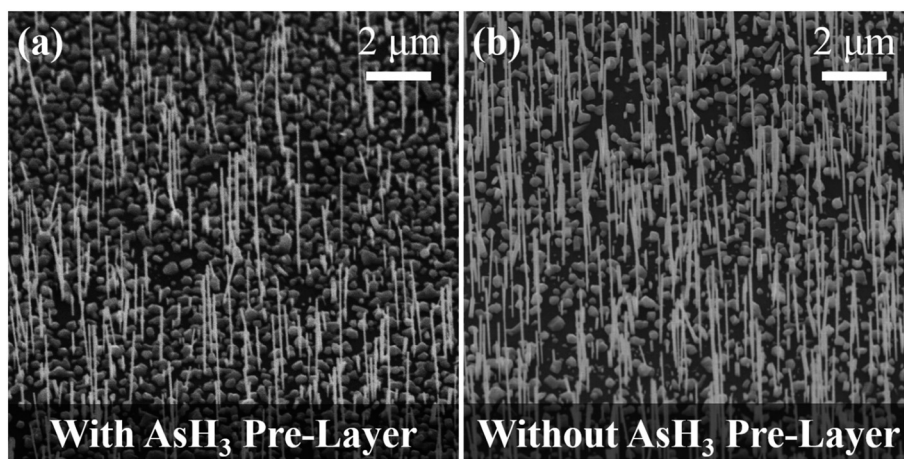
Fig. 6 45° tilted-view SEM images of as-grown InAs NWs formed under otherwise constant conditions, but (a) with and (b) without the use of a pre-growth \text{AsH}_3 surface treatment.
