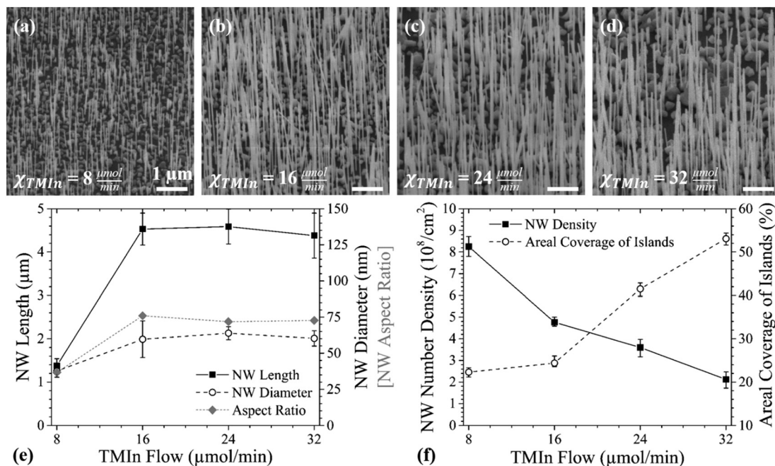
Fig. 3 Flow rate dependence: 45° tilted-view SEM images of as-grown InAs NWs on SLG at \chi_{\text{TMin}} of (a) 8\ \mu\text{mol min}^{-1} , (b) 16\ \mu\text{mol min}^{-1} , (c) 24\ \mu\text{mol min}^{-1} , and (d) 32\ \mu\text{mol min}^{-1} , under constant T_G = 650^\circ\text{C} and V/III = 25. All scale bars represent 1 \mu\text{m} . Measured values for (e) NW height, diameter, and aspect ratio and (f) NW number density and parasitic island areal coverage are plotted as a function of \chi_{\text{TMin}} .
