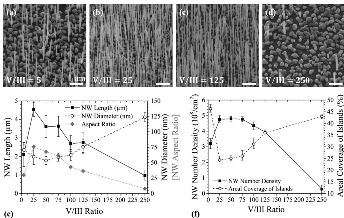
Fig. 1 V/III ratio dependence: 45^\circ tilted-view SEM images of as-grown InAs NWs on SLG at V/III ratio of (a) 5, (b) 25, (c) 125, and (d) 250, under constant T_G = 650^\circ\text{C} and \chi_{\text{TMin}} = 16\ \mu\text{mol min}^{-1} . All scale bars represent 1\ \mu\text{m} . (e) Measured values for NW length (black square data points with solid black line), diameter (white circle data point with dashed black line), and aspect ratio (grey diamond data points with dotted grey line), and (f) NW number density (black square data point with solid black line) and areal coverage of polycrystalline islands (white circle data points with dashed black line), plotted as a function of V/III ratio.
