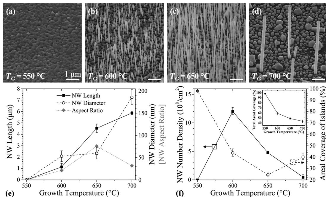
Fig. 2 Temperature dependence: 45° tilted-view SEM images of as-grown InAs NWs on SLG at T_G of (a) 550 °C, (b) 600 °C, (c) 650 °C, and (d) 700 °C, under constant V/III = 25, and \chi_{\text{TMin}} = 16 \mu\text{mol min}^{-1} . All scale bars represent 1 \mu\text{m} . Measured values for (e) NW height, diameter, and aspect ratio and (f) NW number density and parasitic island areal coverage are plotted as functions of T_G . Inset of (f) shows total areal coverage of both NWs and parasitic islands as a function of T_G .
