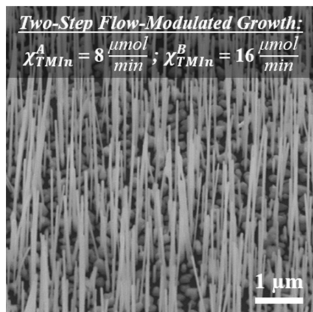
Fig. 7 45° tilted-view SEM image of high aspect ratio and high number density InAs NWs grown using a two-step flow-modulated sequence.
