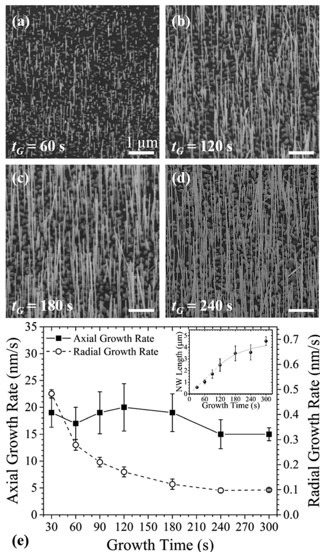
Fig. 5 Growth evolution of NWs under the selected optimal conditions of V/III = 25, T_G = 650^\circ\text{C} , and \chi_{\text{TMin}} = 16 \mu\text{mol min}^{-1} . (a–d) Show 45^\circ tilted-view images after growth durations of 60 s, 120 s, 180 s, and 240 s, respectively. All scale bars represent 1 μm. (e) NW axial growth rates (black square data points with solid black line) and NW radial growth rates (white circle data points with dashed black line) are plotted for various total growth times between 30 s and 300 s. The inset in (e) shows a plot of measured mean NW length versus growth time to demonstrate the growth rate saturation effect; a linear trend near the origin ( i.e. , dashed grey line for t_G \leq 120 s) is used to demonstrate the absence of a significant incubation phase prior to NW formation.
