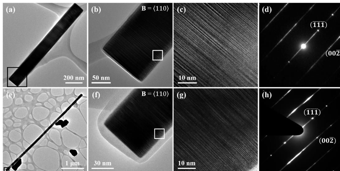
Fig. 4 TEM images obtained along the \langle 110 \rangle zone axis (a–c and e–g) and corresponding SAED patterns (d and h) obtained from two different NWs both grown at T_G = 650^\circ\text{C} . The NW captured in (a–d) was formed at high V/III ratio of 250, but at the optimal \chi_{\text{TMin}} = 16 \mu\text{mol min}^{-1} . The NW shown in (e–h) was formed at the optimal V/III ratio of 25, but at high \chi_{\text{TMin}} = 32 \mu\text{mol min}^{-1} . The highlighted regions in (a, b, e and f) are shown at higher magnification in subsequent panels.
