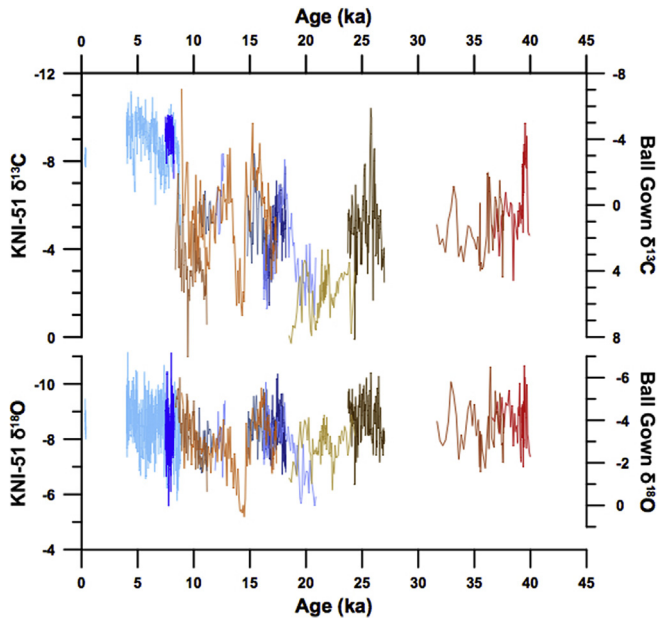
Fig. 2. Kimberley composite stalagmite record carbon and oxygen time series. Ball Gown (right axis; earth tones) and KNI-51 (left axis; blues) stalagmite carbon (top) and oxygen (bottom) time series. Note the different scales on the right and left axes, which reflect site-specific controls on speleothem isotopic ratios. Stalagmites from each cave exhibit similar isotopic values and trends, which allows them to be visually integrated into a single time series. (For interpretation of the references to colour in this figure legend, the reader is referred to the web version of this article.)
