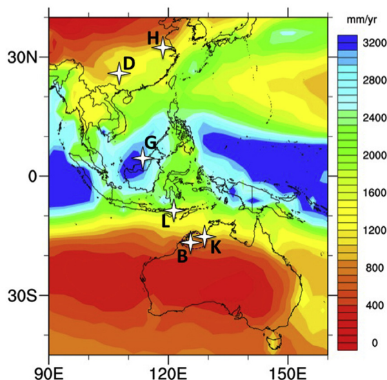
Fig. 1. Total mean annual precipitation for Southeast Asia, the Indo-Pacific, and Australia (1979–2015).
