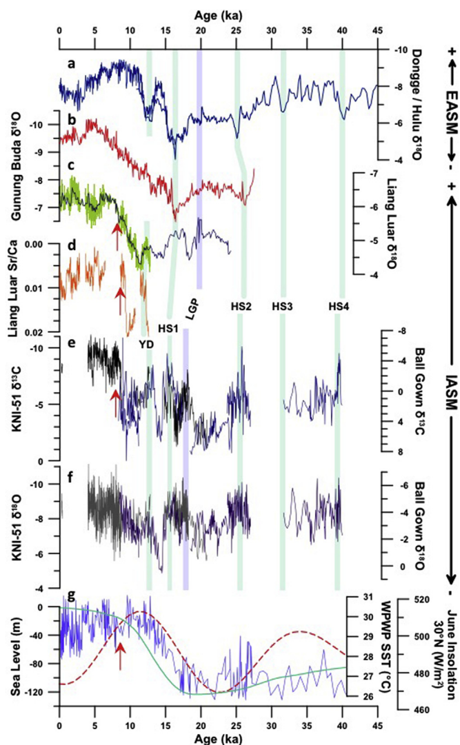
Fig. 4. Kimberley composite stalagmite isotopic records and regional comparisons. a–f. North-to-south array of stalagmite reconstructions of the Austral-Asian monsoon. a. Oxygen isotopic ratios of Dongge cave (Dykoski et al., 2005; dark blue) and Hulu cave stalagmites (Wang et al., 2001; lighter blue); b. Oxygen isotopic ratios from Gunung Buda, Borneo stalagmites (Partin et al., 2007); c–d. Oxygen isotopic (c) and Sr/Ca ratios (d) from Liang Luar, southern Indonesia (Griffiths et al., 2009 – green; Ayliffe et al., 2013 – blue); e–f. KNI-51 (black and grey) and Ball Gown (blue and purple) carbon (e) and oxygen (f) isotopic time series. Isotopic ratios for Ball Gown and KNI-51 are presented on different axes in order to allow the visual integration of the two time series, each of which is influenced by cave-specific controls; g. Eustatic sea level (cyan line; Bintanja and van de Wal, 2008), Indo-Pacific sea surface temperature (purple line; Stott et al., 2002), and June insolation (dashed red line; Berger and Loutre, 1991). Also shown are Heinrich stadials (HS; vertical blue lines), the Younger Dryas (YD), and the Late Glacial Pluvial period (LGP; vertical purple line) identified in the Indonesian and Kimberley records. Gunung Buda record identifies the Antarctic Cold Reversal and not the YD, but neither was demarcated in the figure for ease of interpretation. Similarly, the LGP does not appear to be expressed in the Gunung Buda or Hulu cave records. Red arrows define early Holocene period of enhanced monsoon rainfall. IASM = Indonesian-Australian summer monsoon; EASM = East Asian summer monsoon. (For interpretation of the references to colour in this figure legend, the reader is referred to the web version of this article.)
