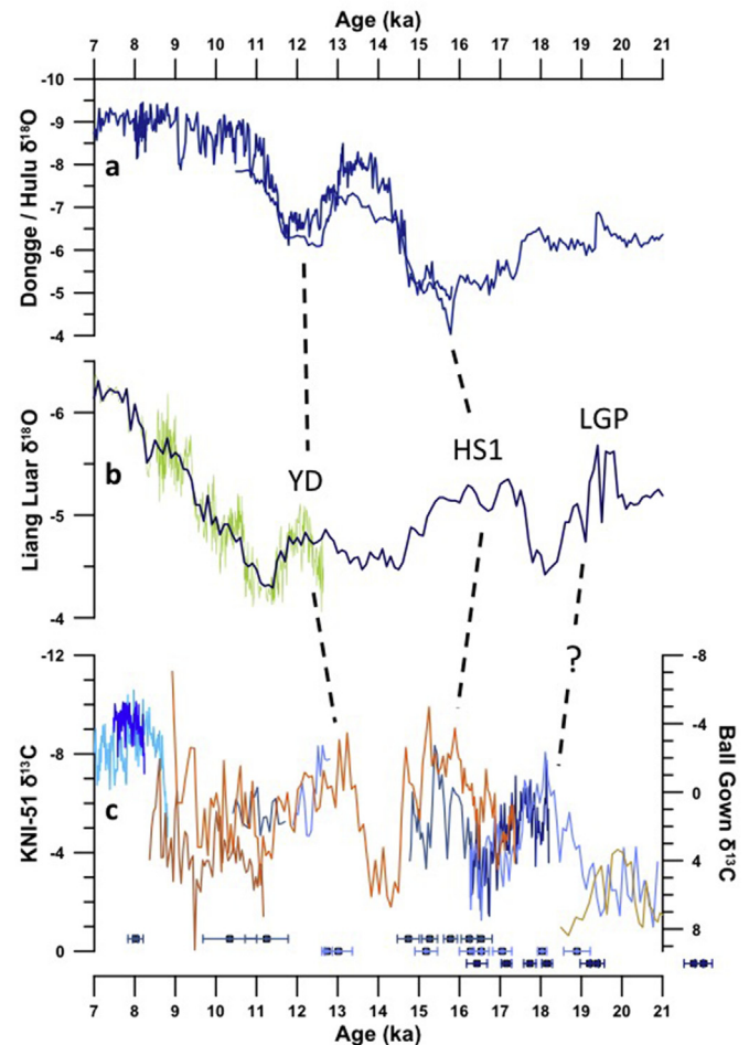
Fig. 3. Late Glacial through early Holocene paleomonsoon variability.
