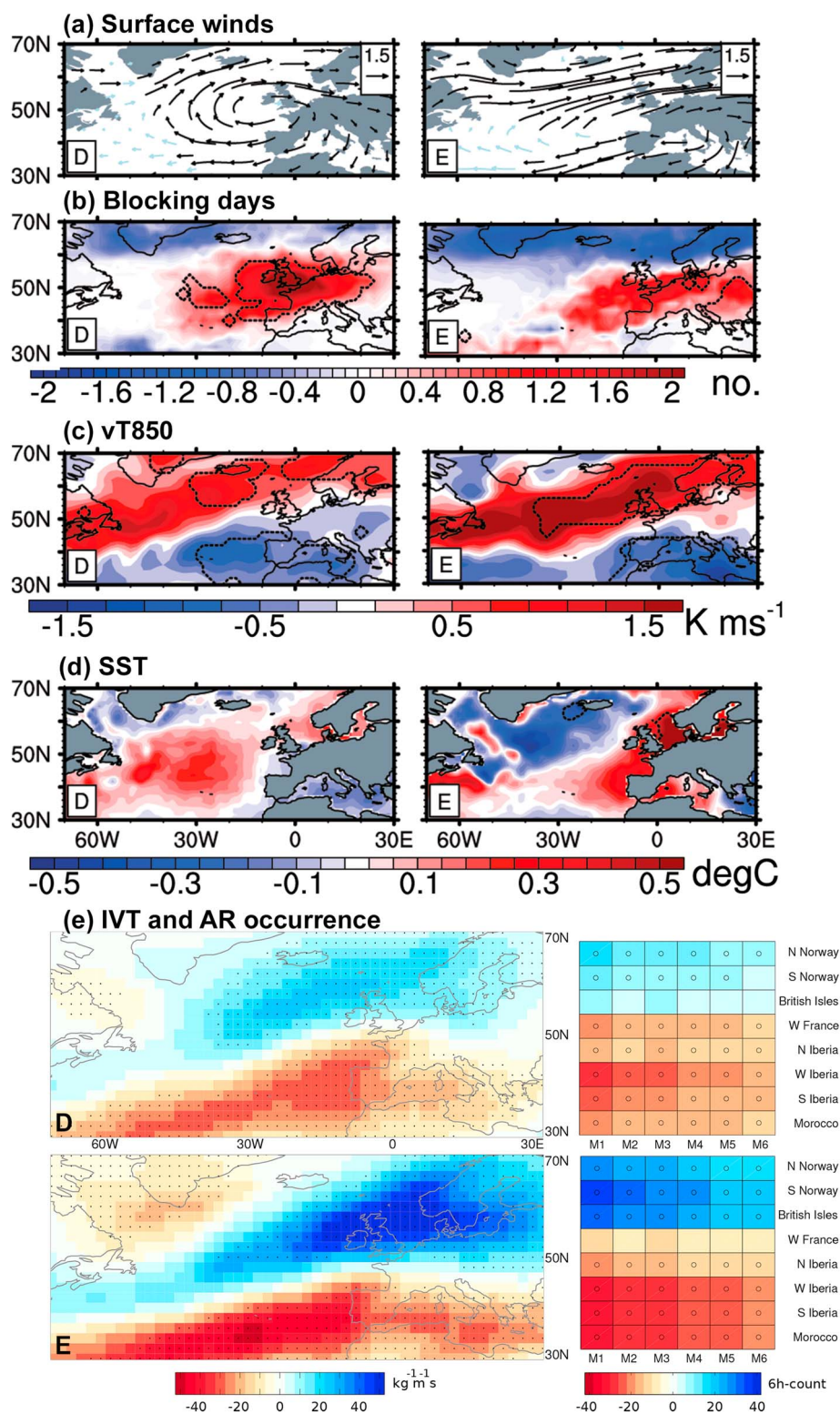
Figure 2. Composite anomalies of (a) surface winds (m/s), (b) number of blocking days per season, (c) 2–6 day band-pass filtered \langle v'T' \rangle at 850 hPa ( \text{K m/s} ), (d) SST ( ^{\circ}\text{C} ), and (e, f) integrated water vapor transport (IVT; \text{kg/m/s} ) and atmospheric river (AR) occurrence, all for JFM for the period 1901–2010 for years in clusters D and E. Count of occurrence of AR events for eight target regions along the eastern Atlantic seaboard. Dashed contours and black vectors in Figures 2a–2d and stippling/circles in Figures 2e and 2f denote anomalies significant at the 2% significance level as estimated by Student's t test. M1 to M6 represent the six method modifications of Brands et al. [2017] using different percentile thresholds to define an AR.
