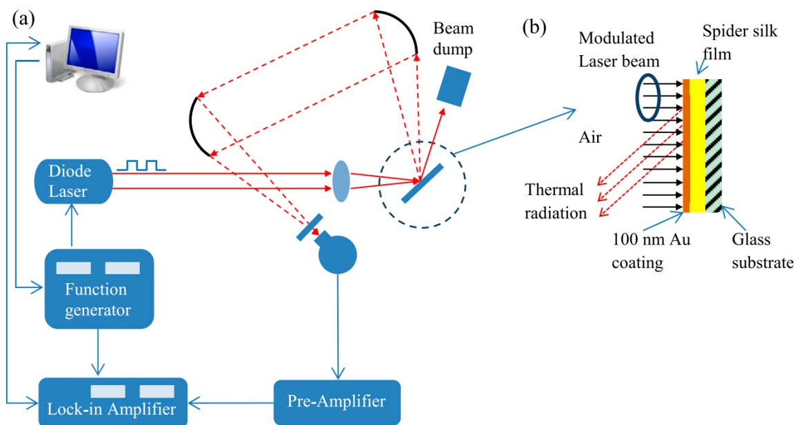
Figure 10. (a) Schematic for photothermal technique (PT) (b) Principle of photothermal technique (PT). Reprinted with permission of the Elsevier [71].
