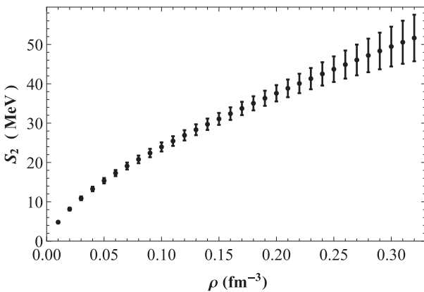
FIG. 13. Isospin-asymmetry energy as a function of the density for the two- and three-body chiral nuclear force models considered in the present work.
