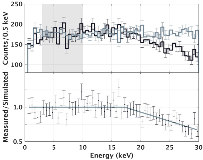
Fig. 6. Top: Comparison of the measured (dark histogram) and simulated (light histogram) ^{133}\text{Ba} calibration spectra, where the initial efficiency hypothesis shown in Fig. 5 has been applied to the latter. The gray shaded region corresponds to the energy range from 3 to 10 keV, which was used to normalize the simulated spectrum to the measured rate. Error bars correspond to 1\sigma -uncertainties. Bottom: Ratio of the measured to simulated energy spectra from the top panel (points), compared to the best-fit, piecewise defined efficiency correction function f(E) (solid line).
