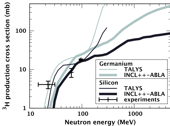
Fig. 1. Tritium production cross sections for neutron spallation on ^{\text{nat}}\text{Ge} and ^{\text{nat}}\text{Si} targets calculated using TALYS version 1.8 [33] and INCL++-ABLA version 5.2.9.5 [36,37]. Results from experiments that measured the tritium production cross section in ^{\text{nat}}\text{Si} are also shown [56–58]. The later calculations in this section use the TALYS cross sections below 100 MeV and the INCL++-ABLA cross sections above 100 MeV.
