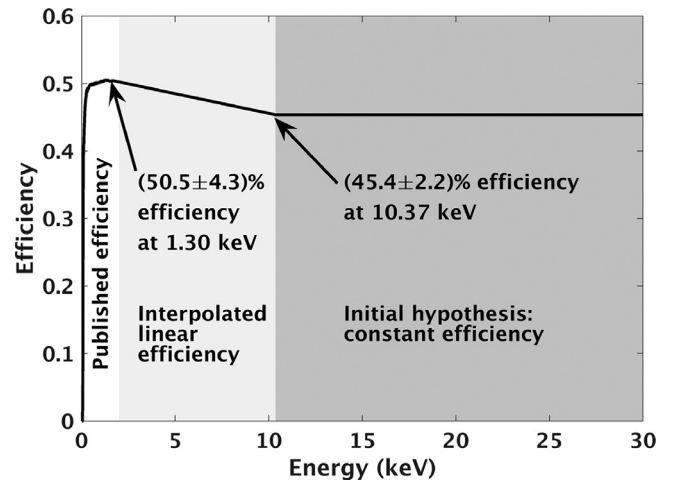
Fig. 5. Initial hypothesis for the CDMSlite detection efficiency as a function of energy (black line). Below 2 keV it matches the published efficiency curve [27] (white region). We linearly interpolate from 2 keV to the value reported in Ref. [27] at 10.37 keV (light grey region). Above 10.37 keV, we use a constant efficiency as our initial estimate (dark grey region).
