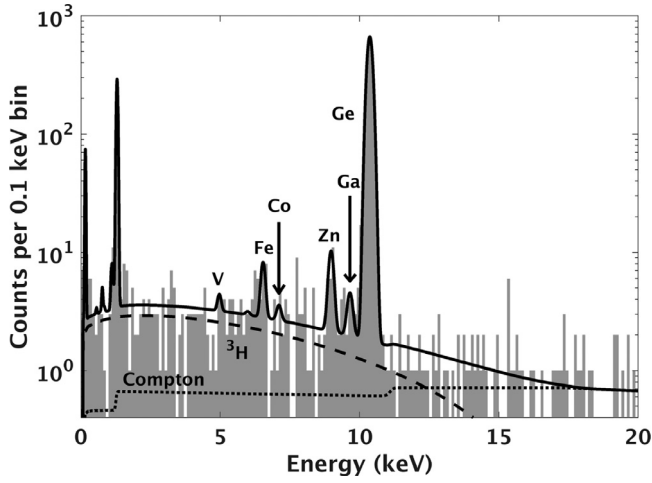
Fig. 8. Maximum likelihood fit to the CDMSlite Run 2 spectrum. The L- and M-shell peaks are not labeled, but occur in the same order as the K-shell peaks.
