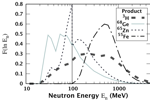
Fig. 3. Calculated probability distribution functions in log-energy for the neutron energy associated with cosmogenic isotope production in ^{\text{nat}}\text{Ge} . These distribution functions, F(\ln E_n) , are given by the product of the cross sections shown in Fig. 2 and the energy-dependent cosmogenic neutron flux. The vertical line indicates the switch from TALYS to INCL-ABLA cross sections.
