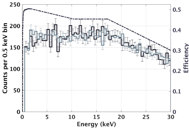
Fig. 7. Comparison of ^{133}\text{Ba} calibration data (dark histogram) with the GEANT4 simulation, corrected by the final efficiency and normalized to the data in the range from 3 to 10 keV (light histogram). Also shown is the final efficiency function (dashed line, right axis).
