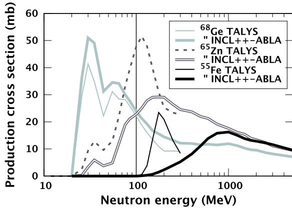
Fig. 2. Calculated production cross sections for neutron spallation on ^{\text{nat}}\text{Ge} using TALYS 1.8 [33] and INCL++-ABLA version 5.2.9.5 [36]. TALYS cross sections are used below 100 MeV (vertical line) and the INCL++-ABLA cross sections above 100 MeV.
