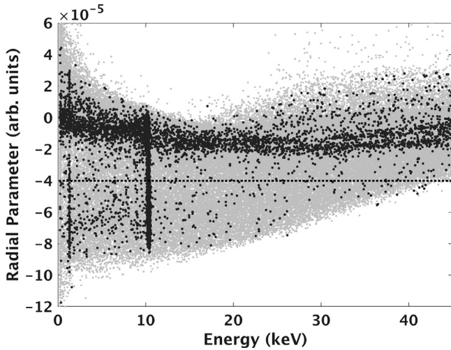
Fig. 4. Radial parameter (for details see Ref. [27]) vs. energy for part of CDM-Slite Run 2, showing dark matter search data (dark points) overlaid on ^{133}\text{Ba} \gamma -calibration data (light grey). Events falling below the radial cut (dotted line) are considered to be within the fiducial volume and are selected for analysis. It is evident that the selection efficiency decreases with increasing energy above \sim 20 keV, which is particularly obvious for the ^{133}\text{Ba} event distribution.
