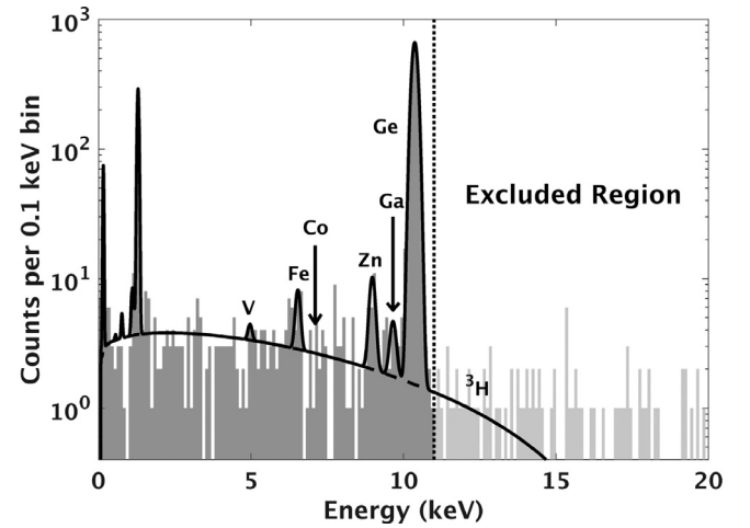
Fig. 10. Maximum likelihood fit neglecting Compton background to determine a conservative upper limit on ^3\text{H} . The fit region is limited to below 11 keV (vertical dotted line) in this case, since the ^3\text{H} spectrum alone cannot reproduce the data at higher energy.
