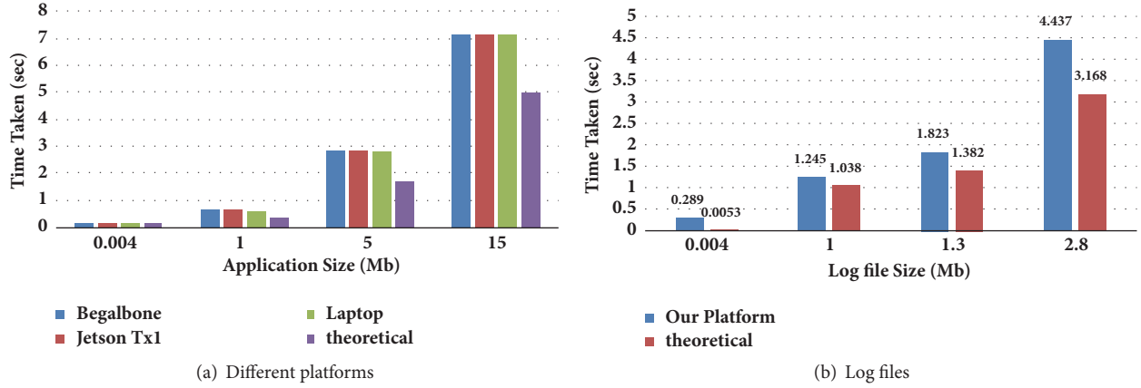
FIGURE 11: (a) The time taken to transfer the application file to the edge node in different hardware platforms and (b) the time taken to transfer the log file from the edge node to the cloud dashboard.
