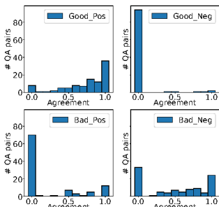
Figure 7: Agreement for the third setting
