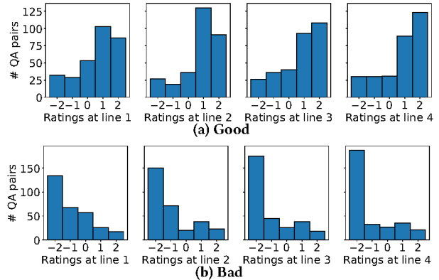
Figure 1: Distribution of confidence ratings from line 1 to 4
