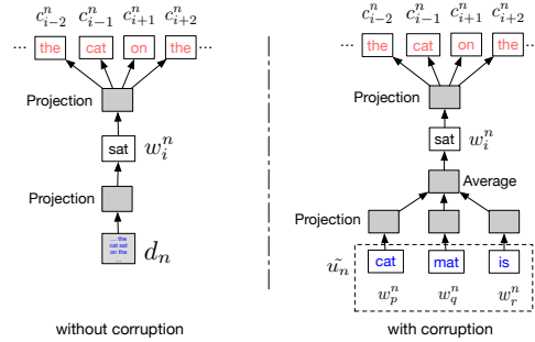
Fig. 1: HDC models used in our experiments. Red words are local context, and blue words are global context.
