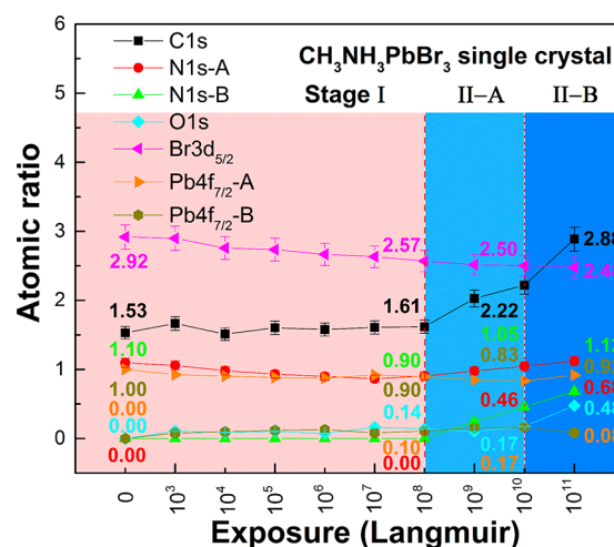
Figure 4. Elemental ratio comparisons of the perovskite single crystal during the water exposures in two stages with error bars.
