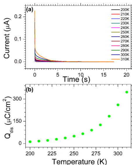
Figure 4. (a) Temperature-dependent discharge currents as a function of time after V = 1.25 V is applied continuously. (b) Corresponding accumulated charge ( Q_{\text{dis}} ) as a function of temperature.
