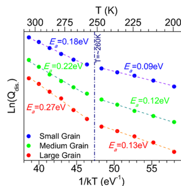
Figure 5. Arrhenius representation of Q_{\text{dis}} obtained from three devices with different average grain sizes upon removal of a continuous voltage of V = 1.25 V.
