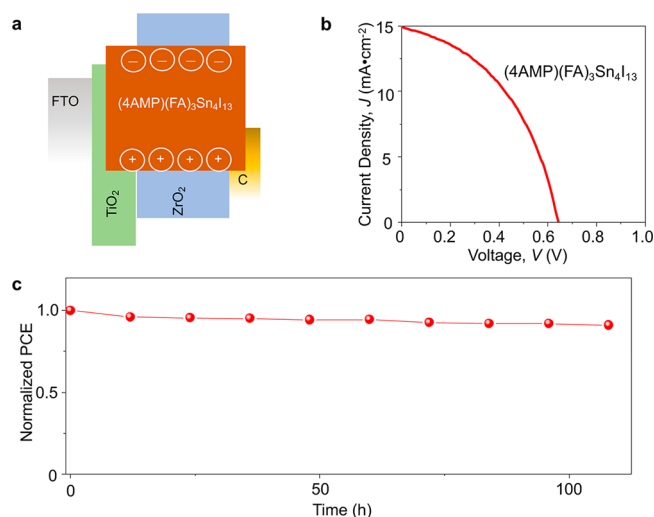
Figure 2. (a) Energy-level diagram for DJ Sn(II)-based HTL-free PSCs. (b) Typical J – V curves for a (4AMP)(FA) 3 Sn 4 I 13 ( n = 4) HTL-free PSCs. (c) PCE stability of a (4AMP)(FA) 3 Sn 4 I 13 -based HTL-free PSC as a function of storage duration (in N 2 atmosphere, at 45 °C, under 1-sun illumination).
