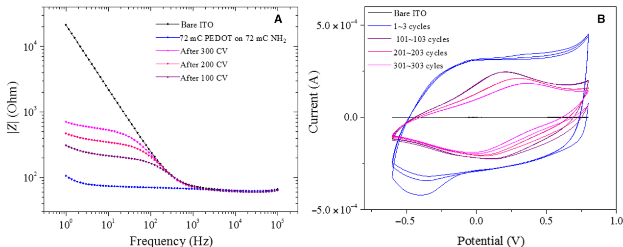
Fig. 9. Electrochemical stability of PEDOT on P(EDOT-NH 2 ). (A) Impedance spectra of 72-mC/cm 2 PEDOT on 72-mC/cm 2 P(EDOT-NH 2 )-coated ITO before and after 100, 200, and 300 cycles of CV scans. (B) CV changes during scanning.
