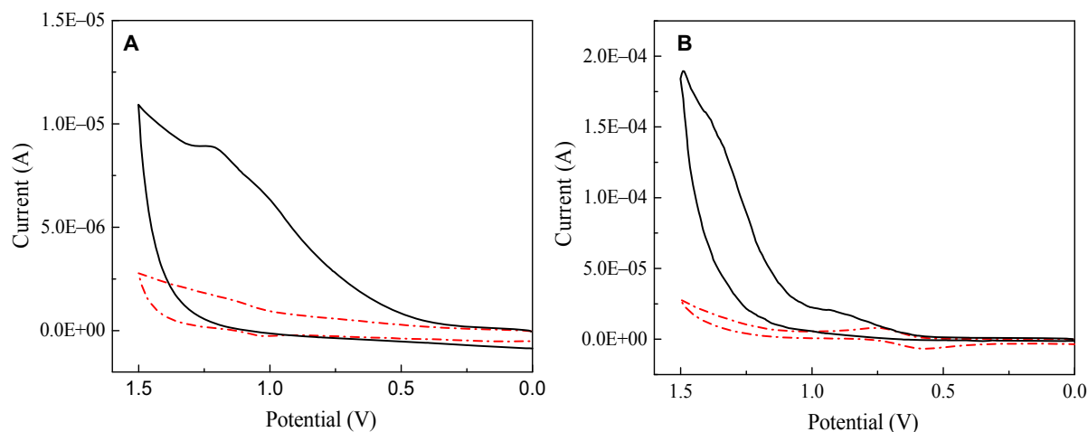
Fig. 2. Wide potential scan in EDOT-NH 2 solution. (A) Pt in EDOT-NH 2 acetonitrile solution with 0.1 M tetrabutylammonium perchlorate (TBAP) as electrolyte (black solid line); Pt in 0.1 M TBAP acetonitrile supporting electrolyte (red dashed line). (B) ITO in EDOT-NH 2 acetonitrile solution with 0.1 M TBAP as electrolyte (black solid line); ITO in 0.1 M TBAP acetonitrile supporting electrolyte (red dashed line). Potential was plotted against the Ag/AgCl pseudoreference electrode (−0.48 V versus ferrocene E 1/2 ).
