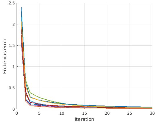
Fig. 2. Frobenius error of the low-rank matrix recovery (vs. iteration number) for different random initializations with (c, p, r) = (15, 20, 3) .
