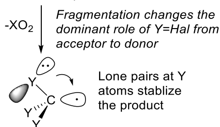
Scheme 1. The chameleonic change of the halogen substituents from \sigma_{C-Y} acceptors to n_Y donors in the process of C-X bond fragmentations
