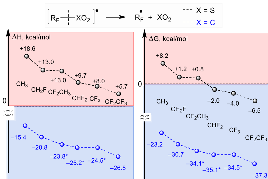
Figure 13: Enthalpies and free energies for the R F -XO 2 (X = S, top, or C, bottom) bond fragmentations in the fluoroalkyl-XO 2 radicals.
