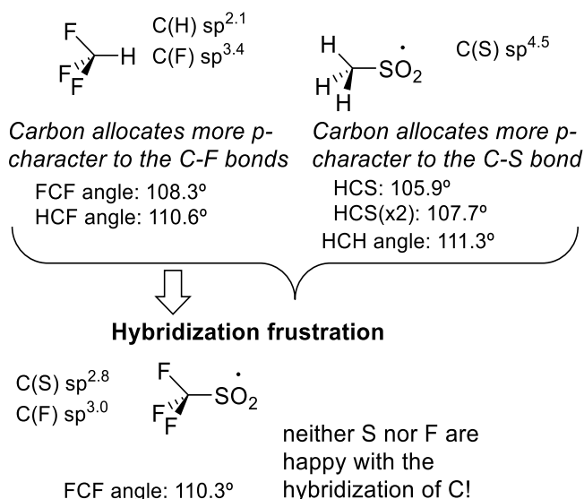
Figure 8: Illustration of “hybridization frustration” in the CF_3SO_2 radical. Average NBO hybridization from the \alpha - and \beta -spin NBOs are given
