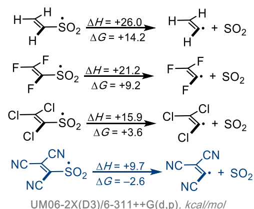
Figure 12: Substituent effects on the BDEs of alkene sulfonyl precursors
