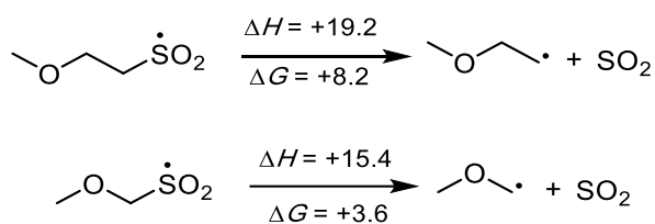
Scheme 2. Evaluation of systems that invoke anomeric stabilization
