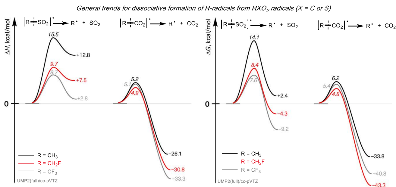
Scheme 4. Effect of fluorine substitution on kinetics and thermodynamics of \text{XO}_2 extrusion from \text{RXO}_2 radicals. ( \text{X}=\text{S},\text{C} )
