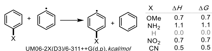
Figure 11: Isodesmic equation evaluating the impact of para -substituted phenyl radicals. Both donor and acceptor groups offer little difference when compared to H.
