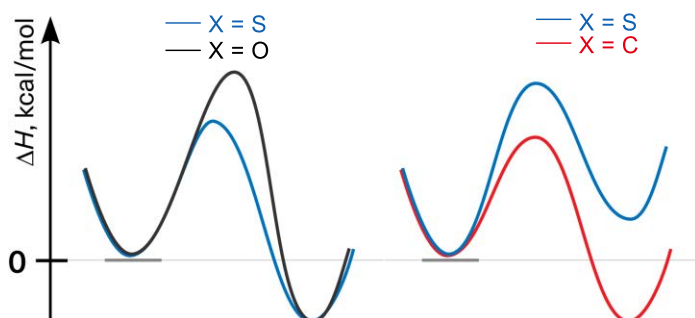
Scheme 5. Comparison of kinetic and thermodynamic trends in fragmentations producing an alkyl radical and a triatomic heterocumulene.
